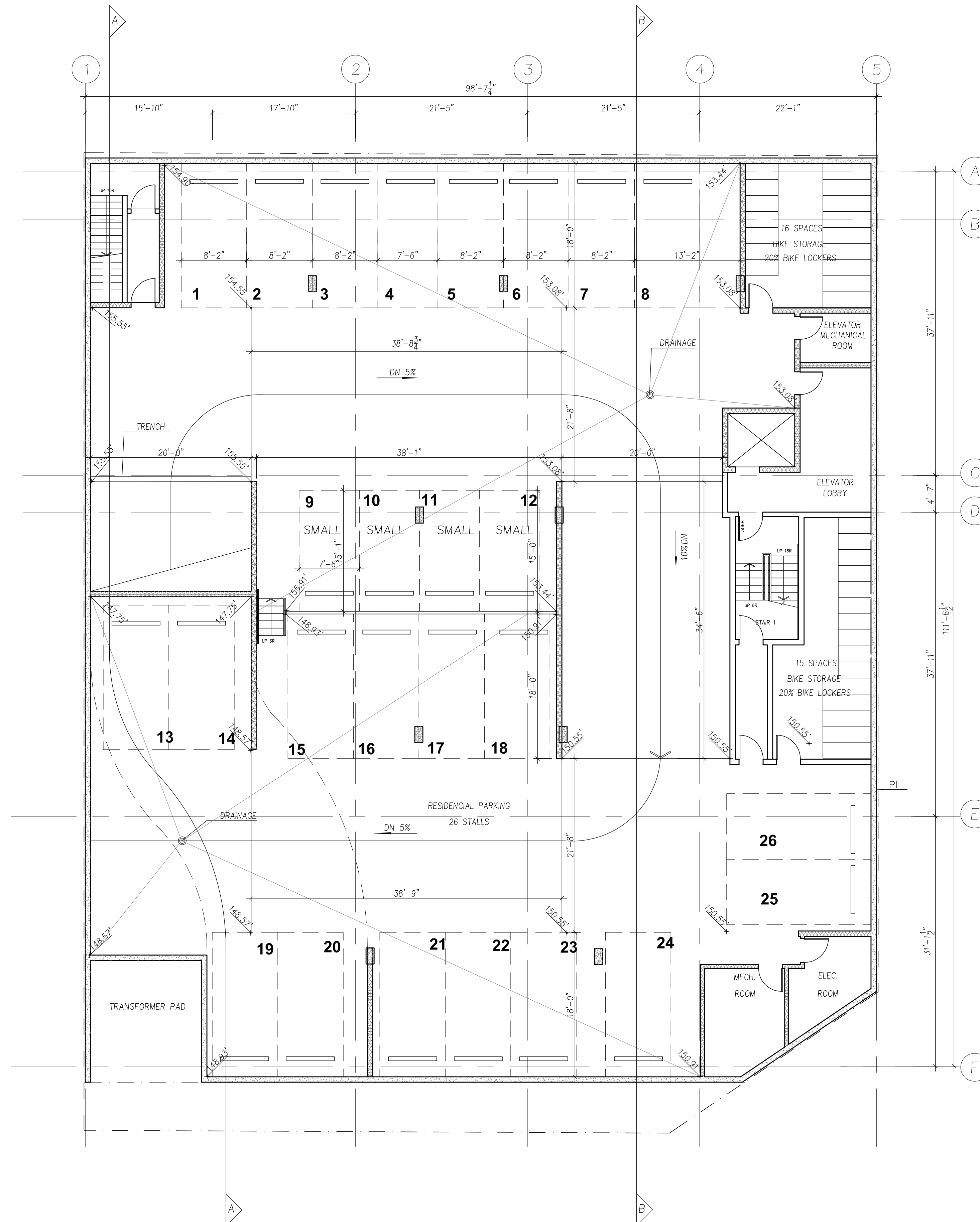
PARKING PLAN
