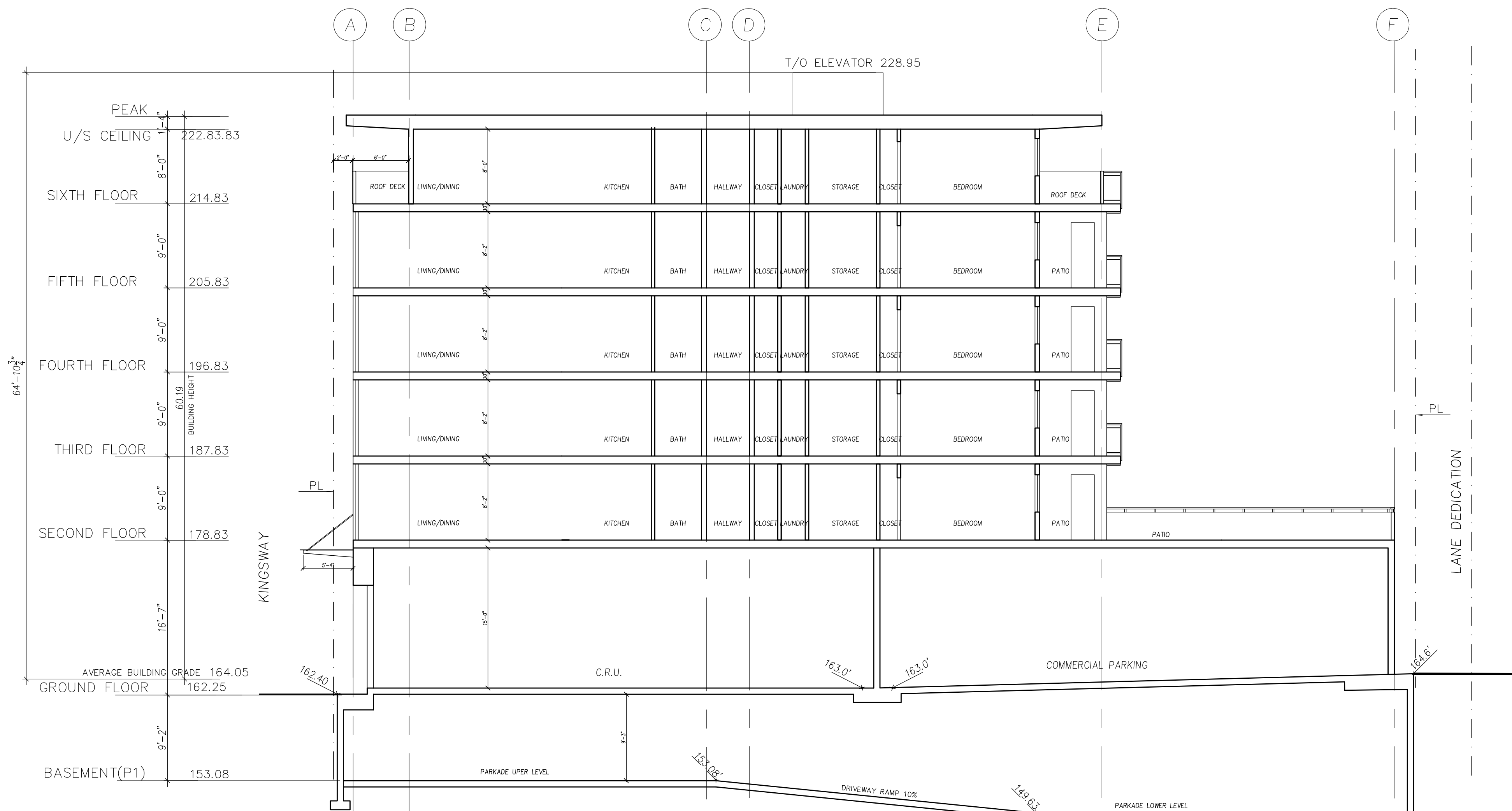
B-B SECTION
