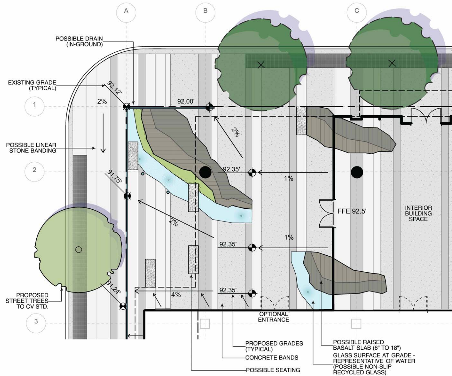
L3 - BLOWUP LEVEL 1 PLAN
