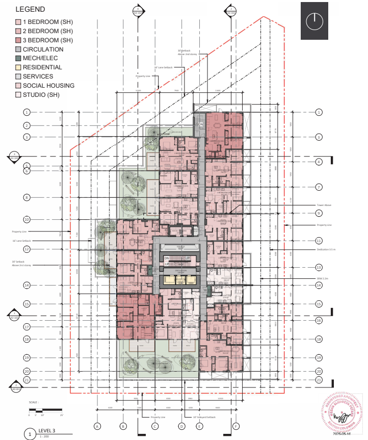
Floor Plan - Level 03 (Social Housing)
