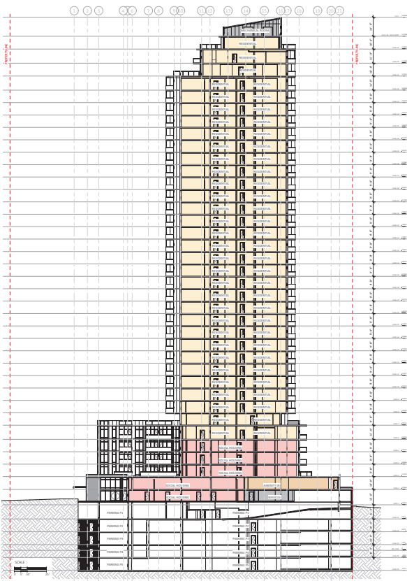
Section C
