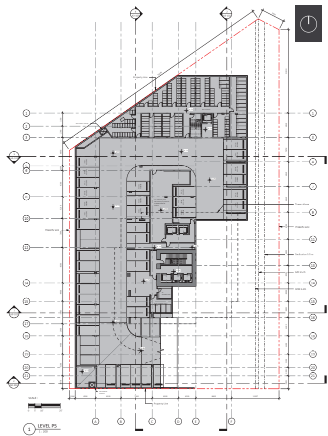
Floor Plan - P5
