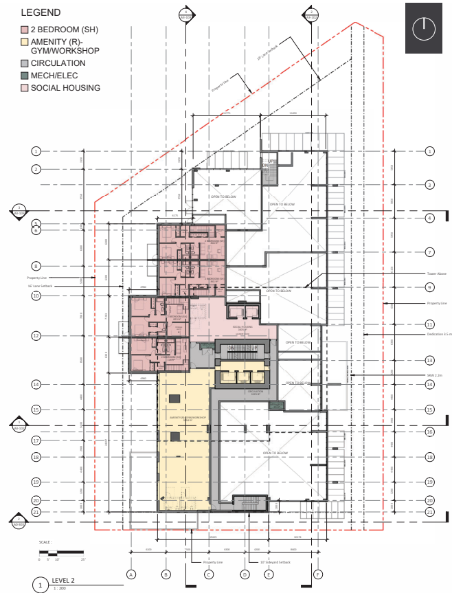
Floor Plan - Level 02 ( Social Housing + Strata Amenity)
