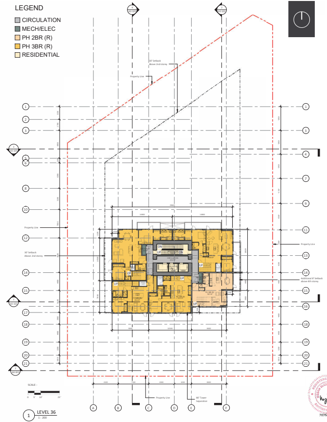
Floor Plan - Level 36 (Strata Residential)
