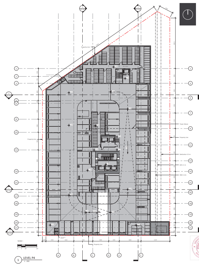
Floor Plan - P4
