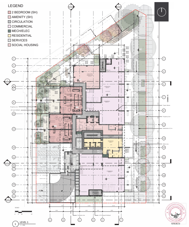
Floor Plan - Level 01 (Social Housing + Commercial)
