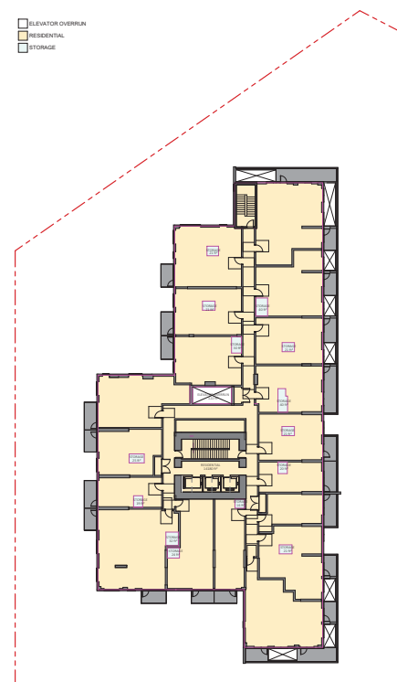
1 LEVEL 6 1:100
