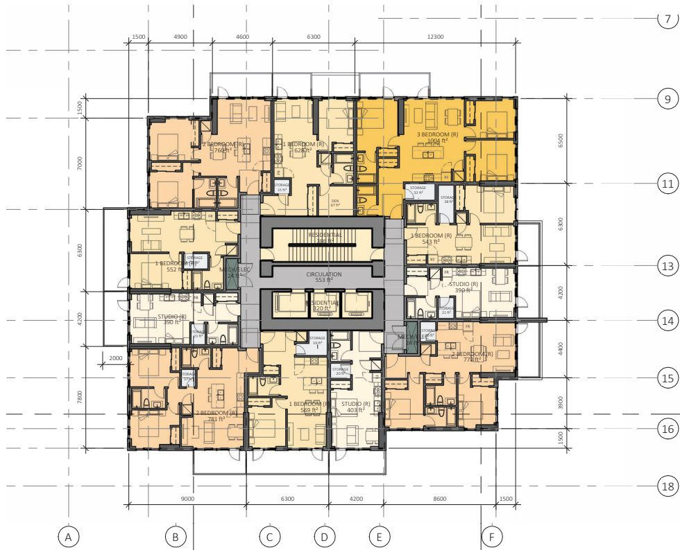
Floor Plan - Level 08 (Typ. Strata Residential) Floor Plate: 8097 sqft
