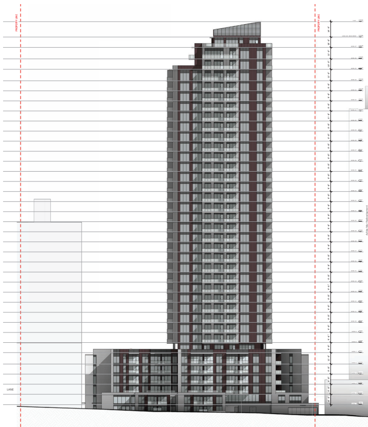
West Elevation
