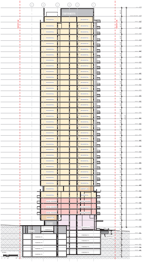
Section B
