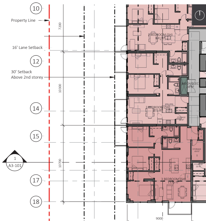
Social Housing 2 Bedroom and 3 Bedroom Units
