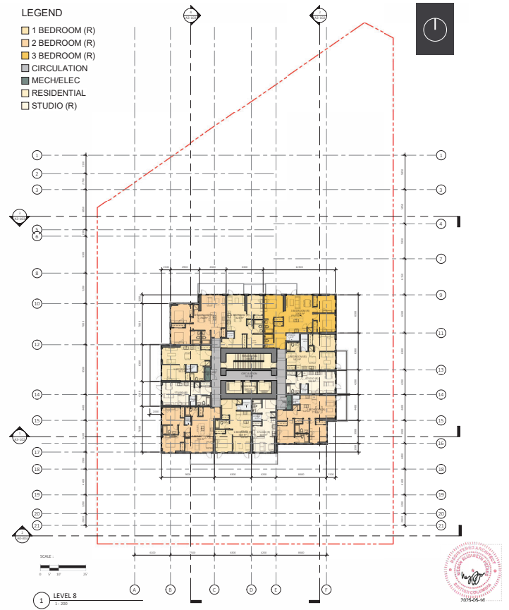
Floor Plan - Level 08 (Typ. Strata Residential Level 08-34)
