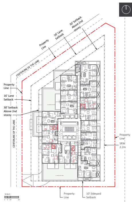
Podium Setbacks
