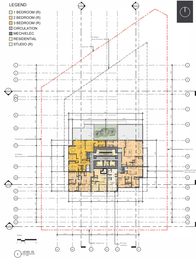
Floor Plan - Level 35 (Strata Residential)
