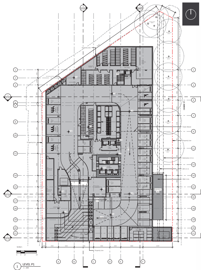
Floor Plan - P1
