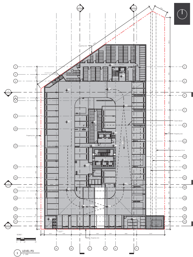
Floor Plan - P3
