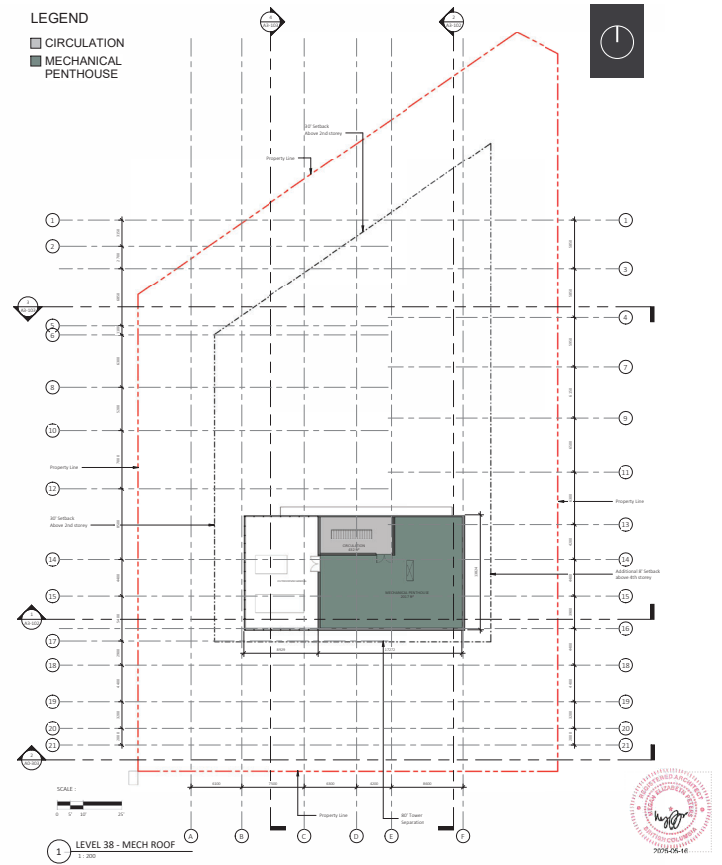
Floor Plan - Level 38 (Mechanical Penthouse)
