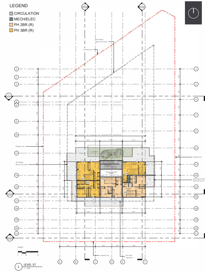
Floor Plan - Level 37 (Strata Residential)
