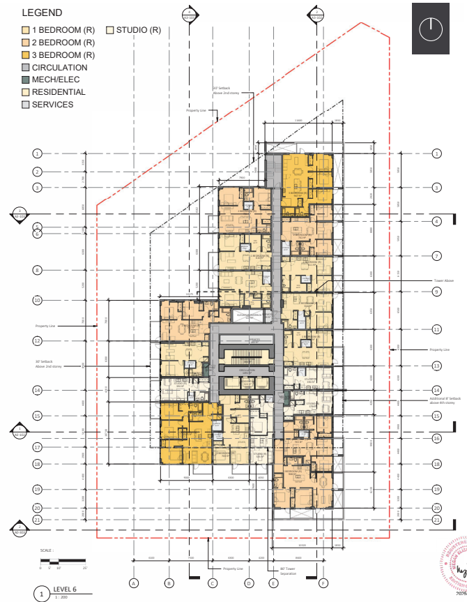
Floor Plan - Level 06 (Social Housing + Strata Residential)
