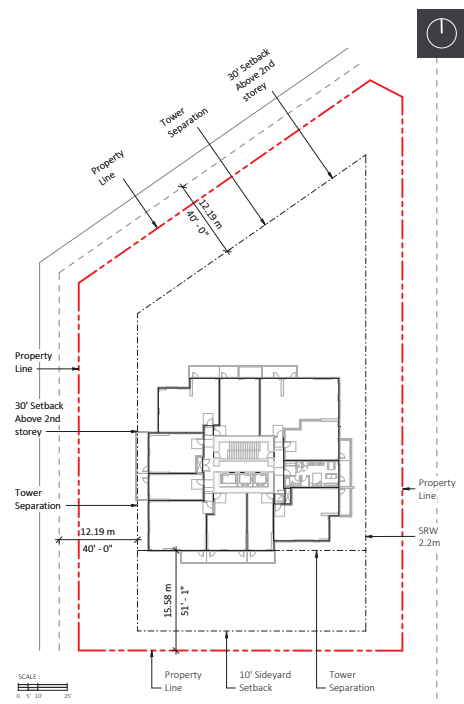
Tower Setbacks
