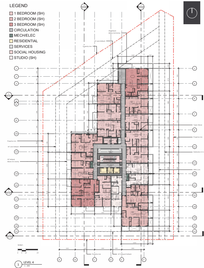
Floor Plan - Level 04-05 (Social Housing)
