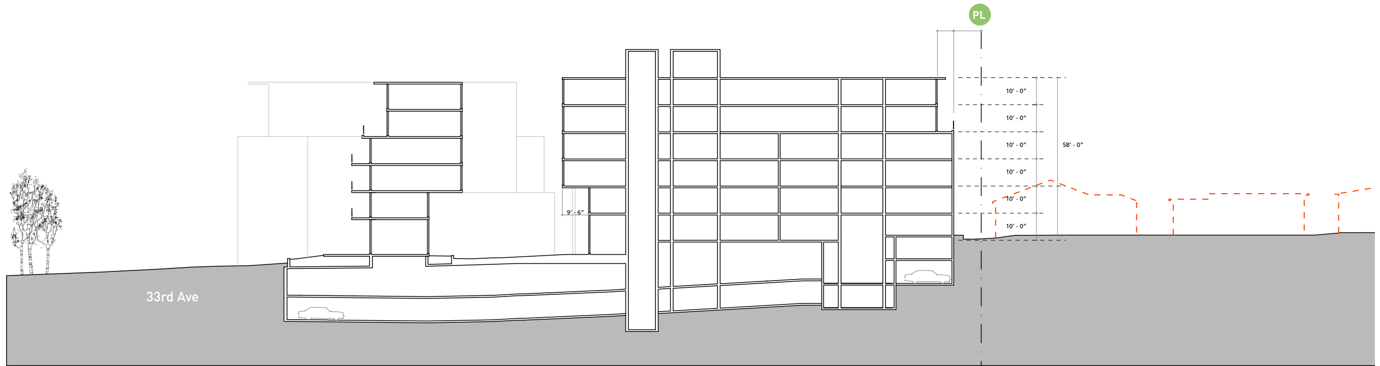
Section CC
