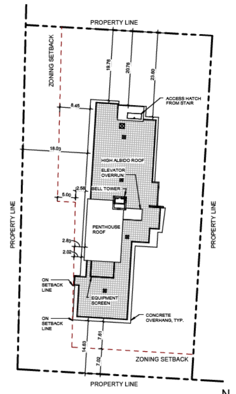
8 UPPER ROOF PLAN SETBACKS A11 1:384
