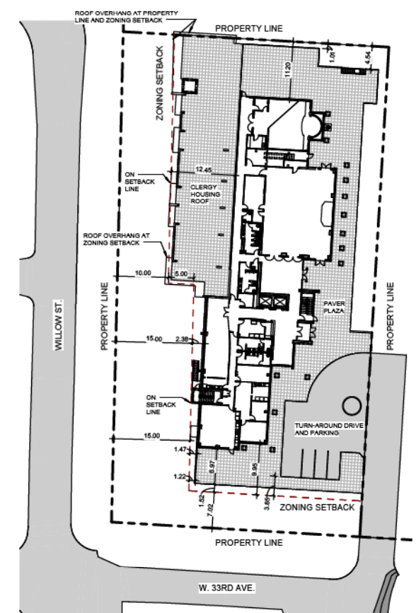
3 LEVEL 1 FLOOR PLAN SETBACKS A11 1:384
