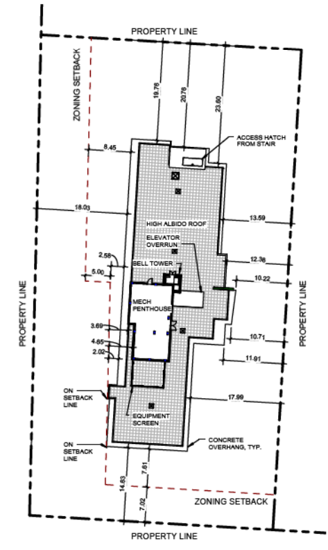
7 PENTHOUSE ROOF PLAN SETBACKS A11 1:384
