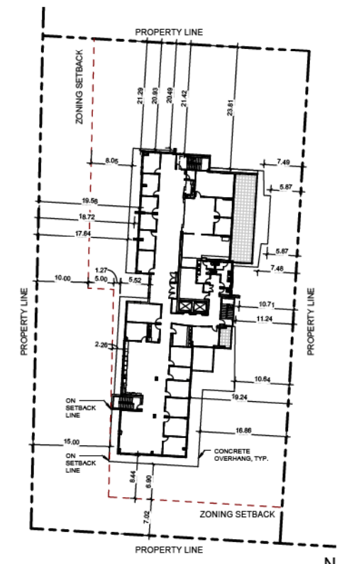
5 LEVEL 3 FLOOR PLAN SETBACKS A11 1:384
