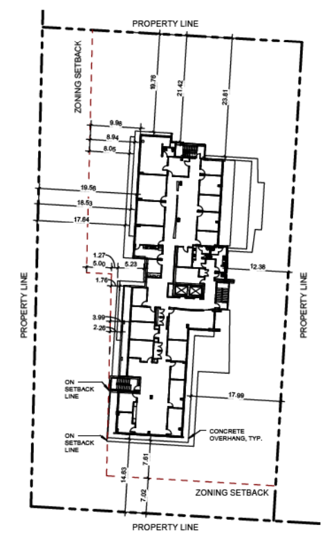
6 LEVEL 4 FLOOR PLAN SETBACKS A11 1:384
