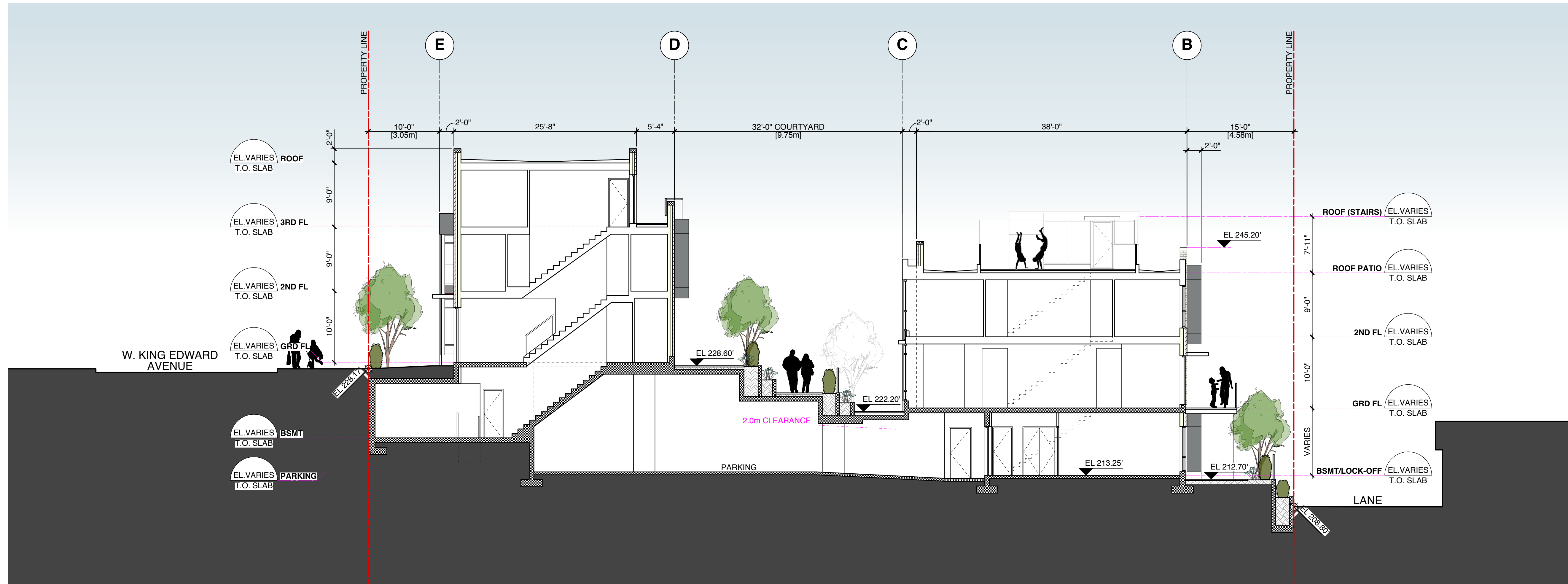
1 BUILDING SECTION
