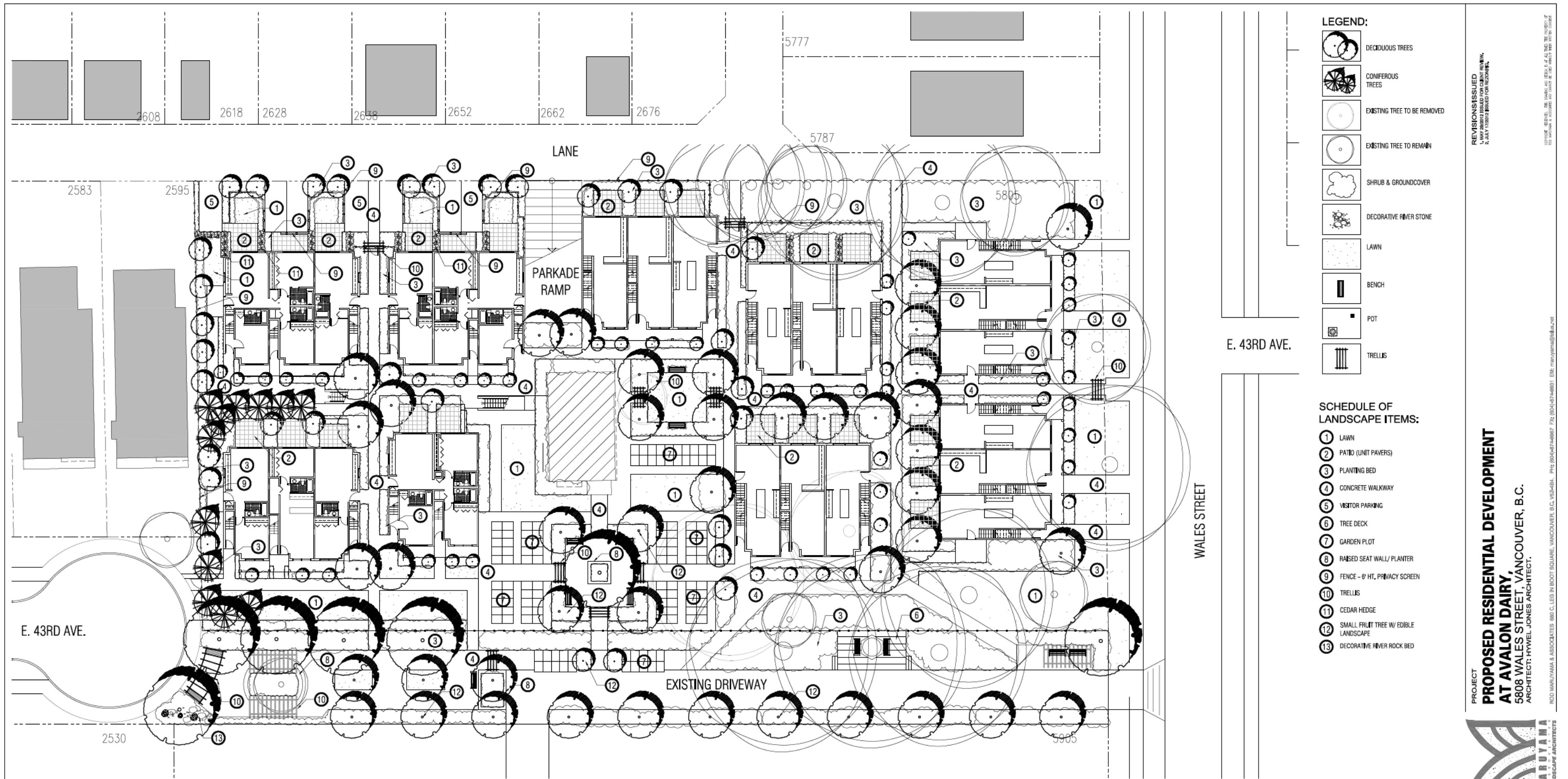
SITE PLAN: LANDSCAPE SCALE: 1/16"=1'-0"
