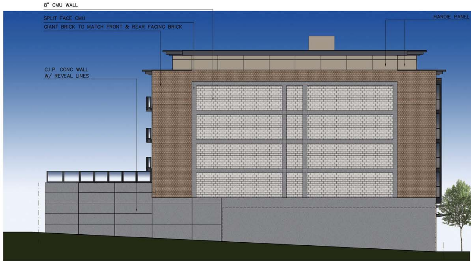
NORTH ELEVATION
