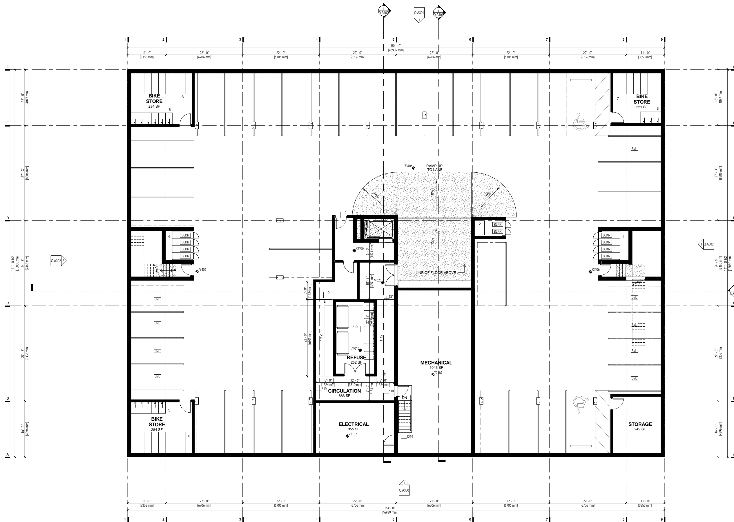
1 Parking - P1 1/8" = 1'-0"
