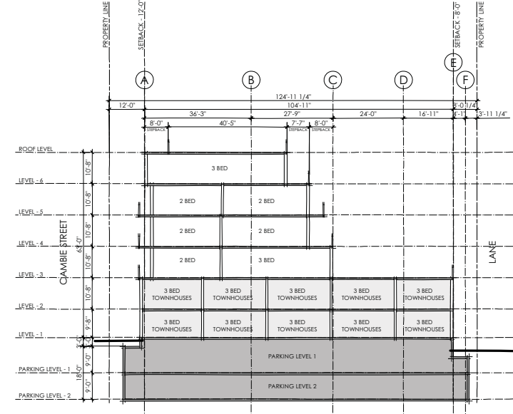
SECTION E-E
