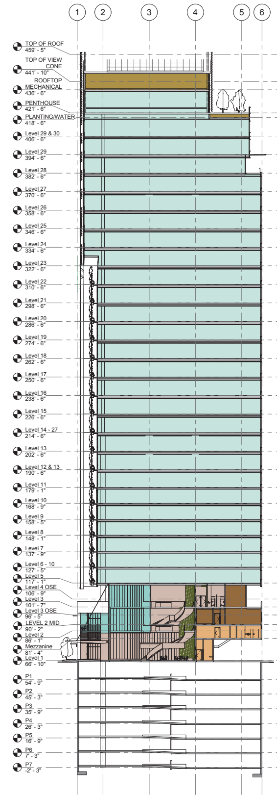
Section B-B
