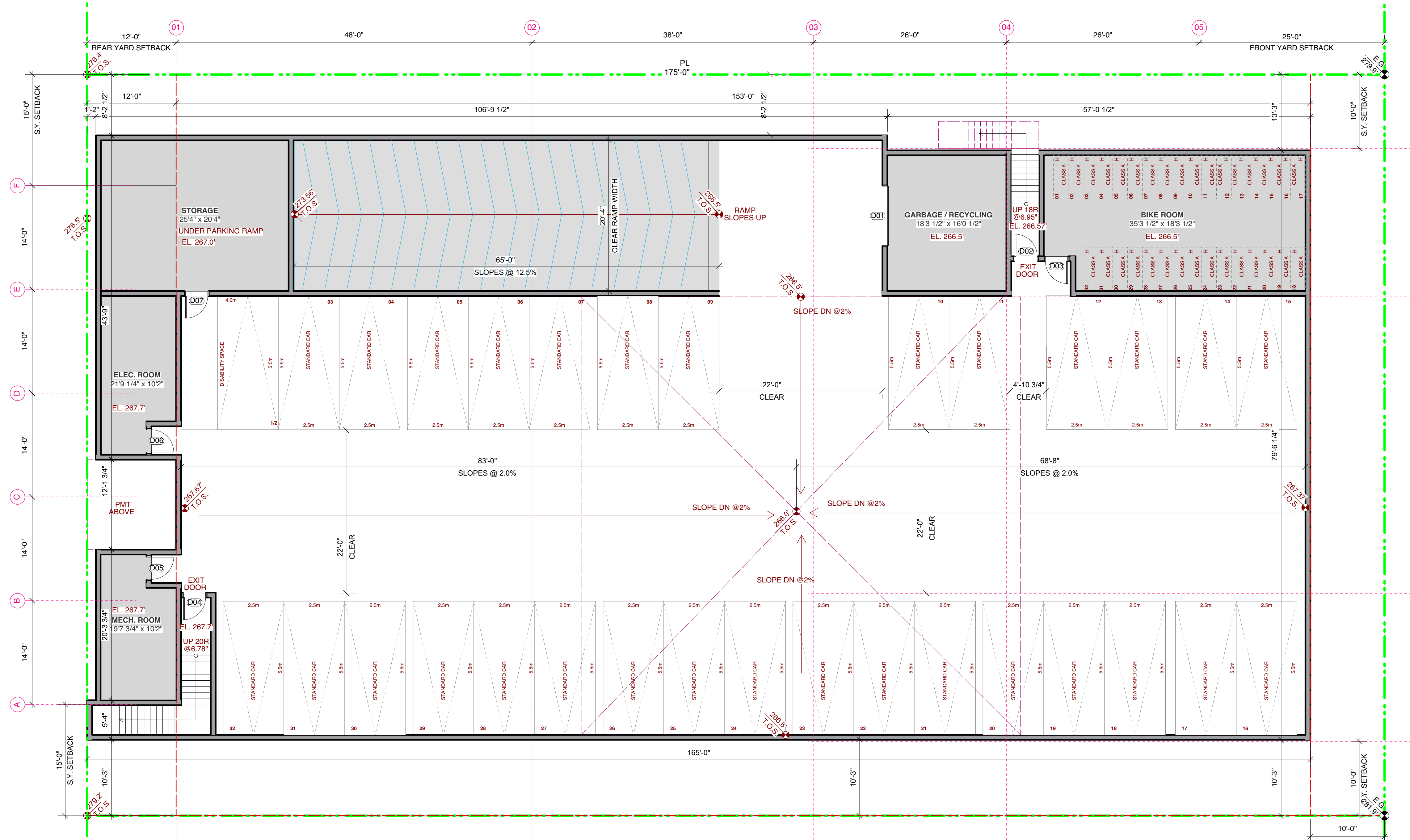
1 Basement Parkade Plan Scale: 1/8" = 1'-0"
