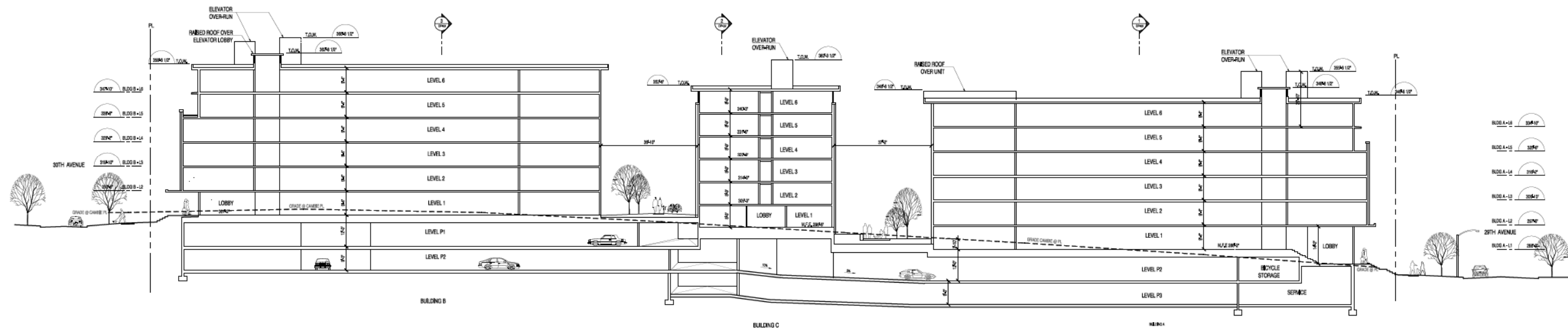
1 SECTION - Lengthwise thru Site SCALE: 1/8"=1'-0"
