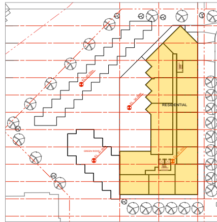
Typical Floor - Level 41.0 m
