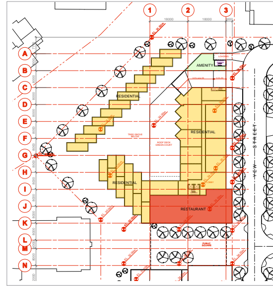
Upper Ground Floor - Level 34.0 m
