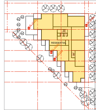
Typical Floor - Levels 37.0, 40.0, 43.0, 46.0 m
