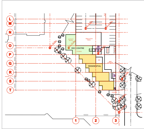
Lower Ground Floor - Level 31.5 m
