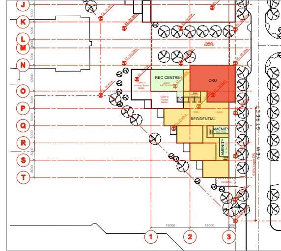
Upper Ground Floor - Level 34.0 m
