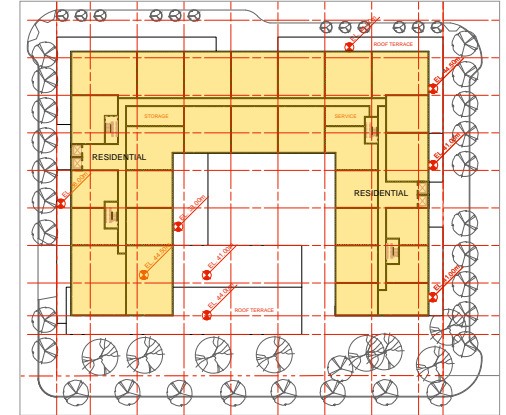
Typical Floor - Levels 44.5, 47.5 m
