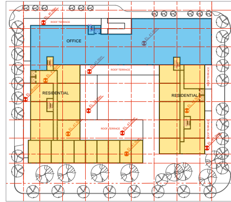
Second Floor - Level 41.0 m
