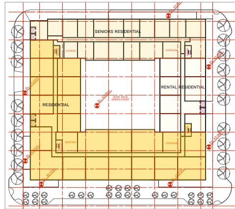
Typical Floor - Levels 43.0, 46.0, 43.0, 52.0 m
