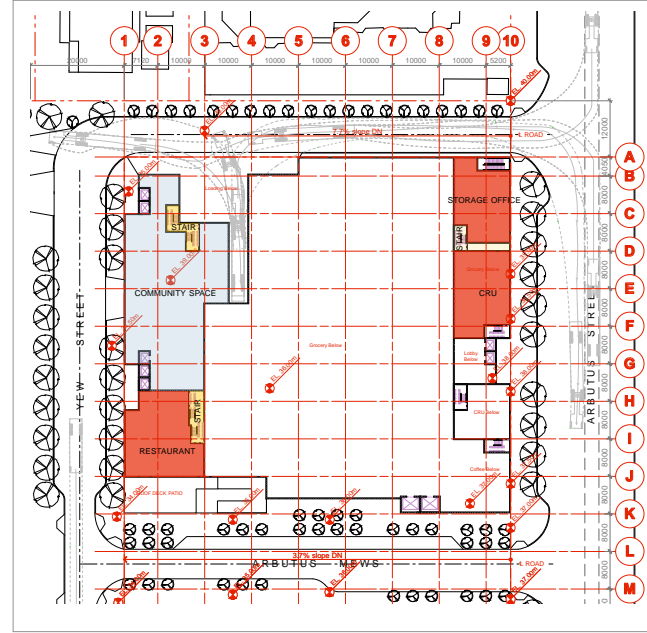
Upper Ground Floor - Level 39.0 m
