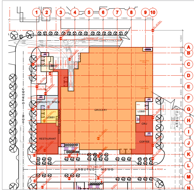
Lower Ground Floor - Level 36.0 m
