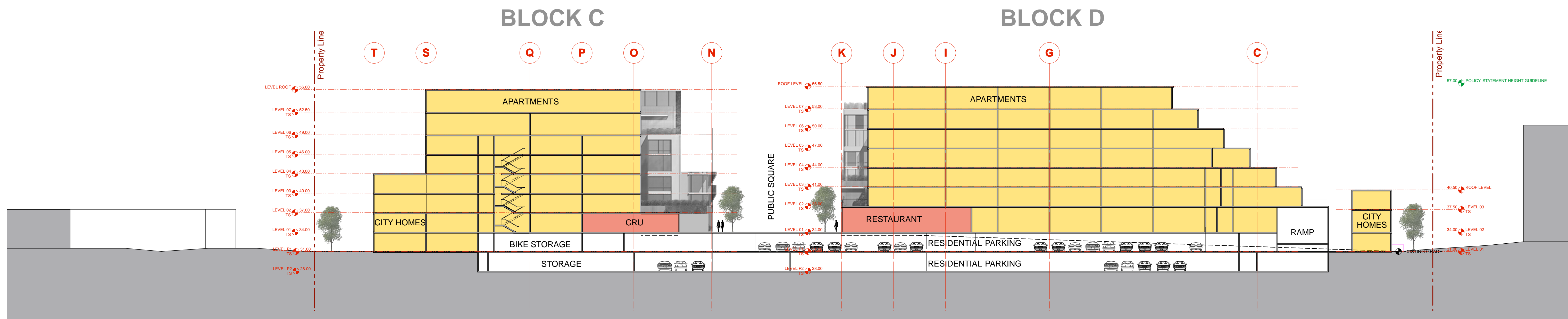
NORTH-SOUTH SECTION THROUGH BLOCKS C&D SCALE: 1:300
