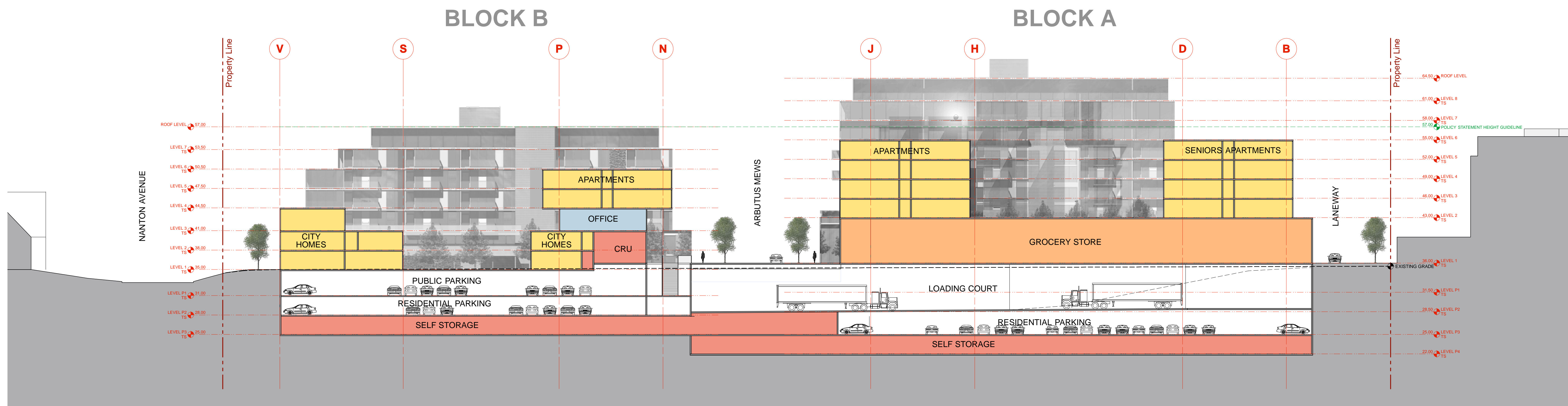
NORTH-SOUTH SECTION THROUGH BLOCKS A&B SCALE: 1:300
