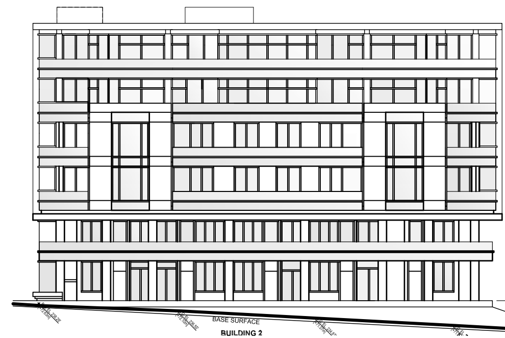
BUILDING 2 - EAST ELEVATION (OLD DESIGN)
