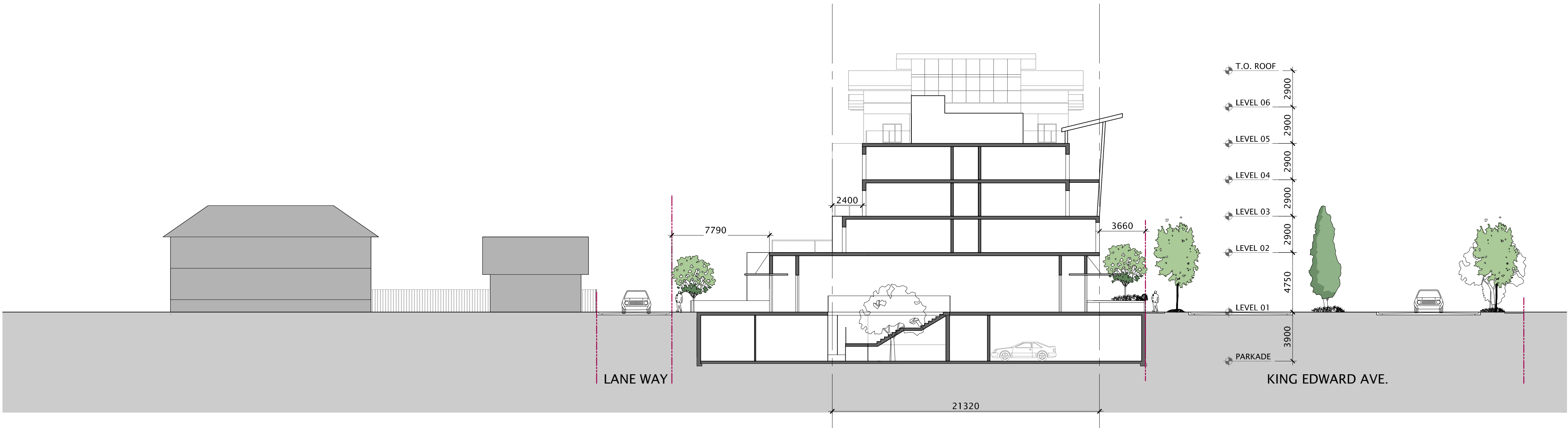
01 A31-01-02 1 : 200 BUILDING SECTION 3 LOOKING WEST
