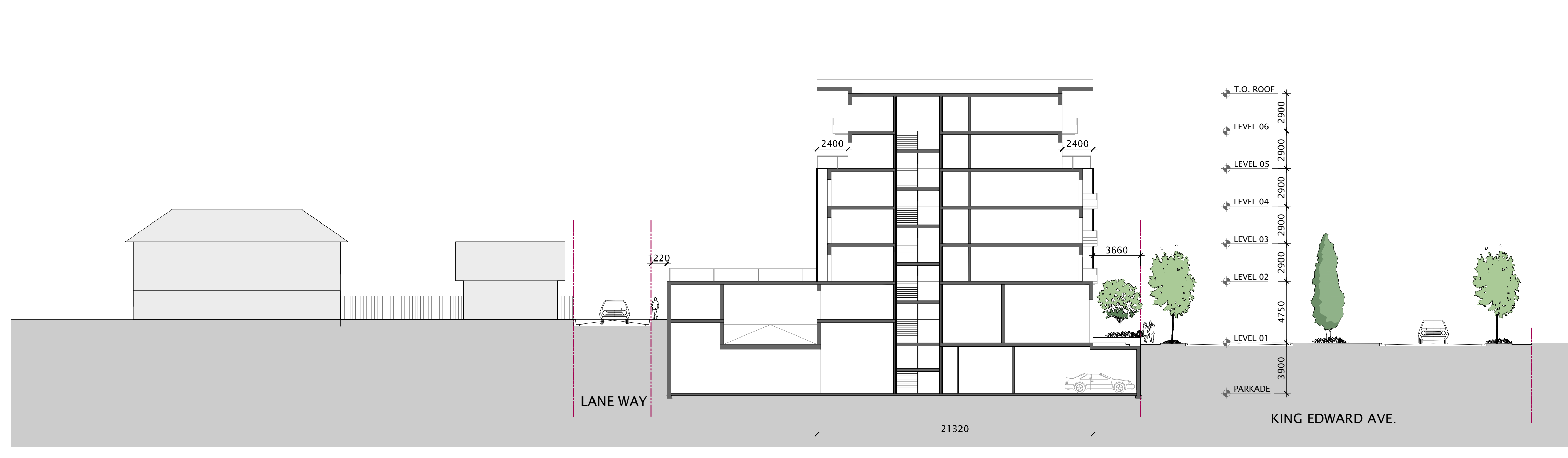
BUILDING SECTION 2 LOOKING WEST 02 A31-01-01 1 : 200
