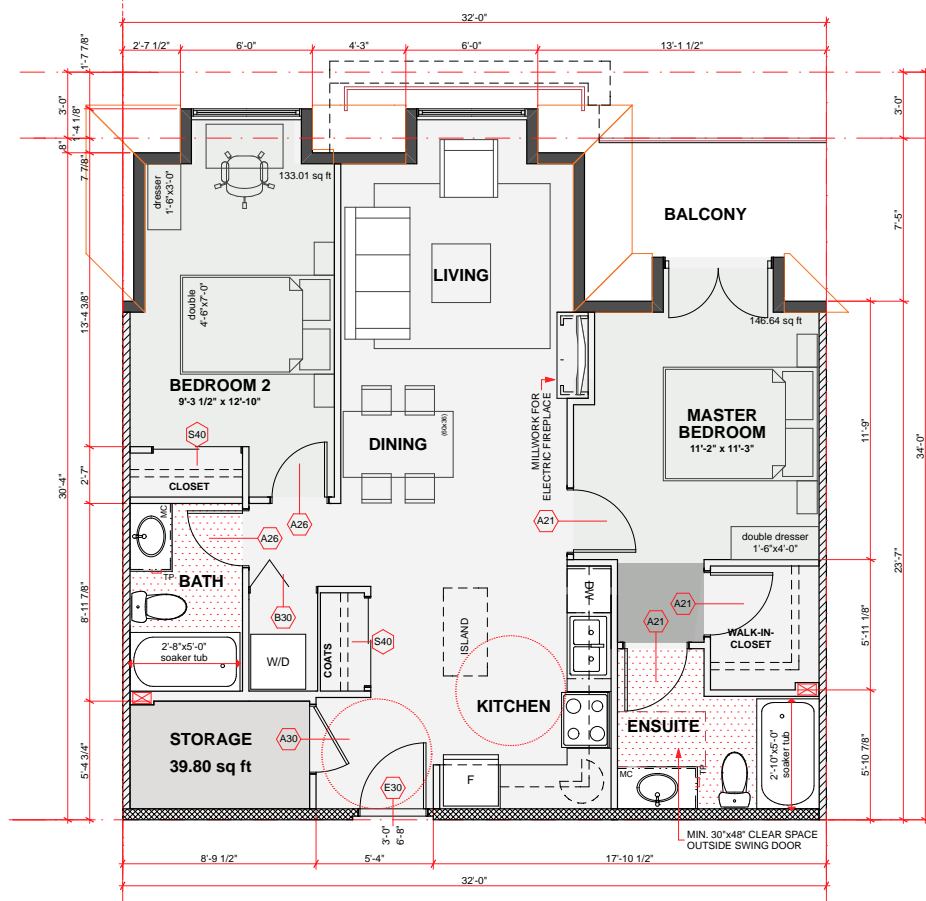
UNIT C-3 2BDRM 928.05 sq
