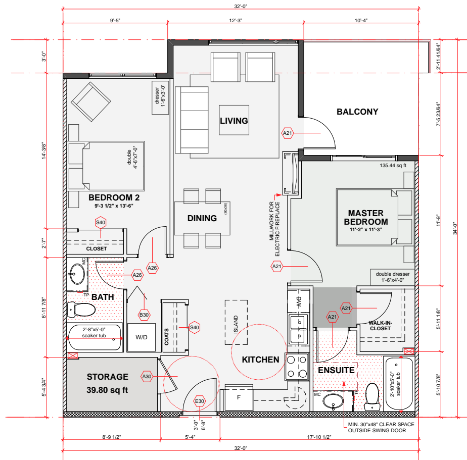
UNIT C-2 2BDRM 952.11 sq
