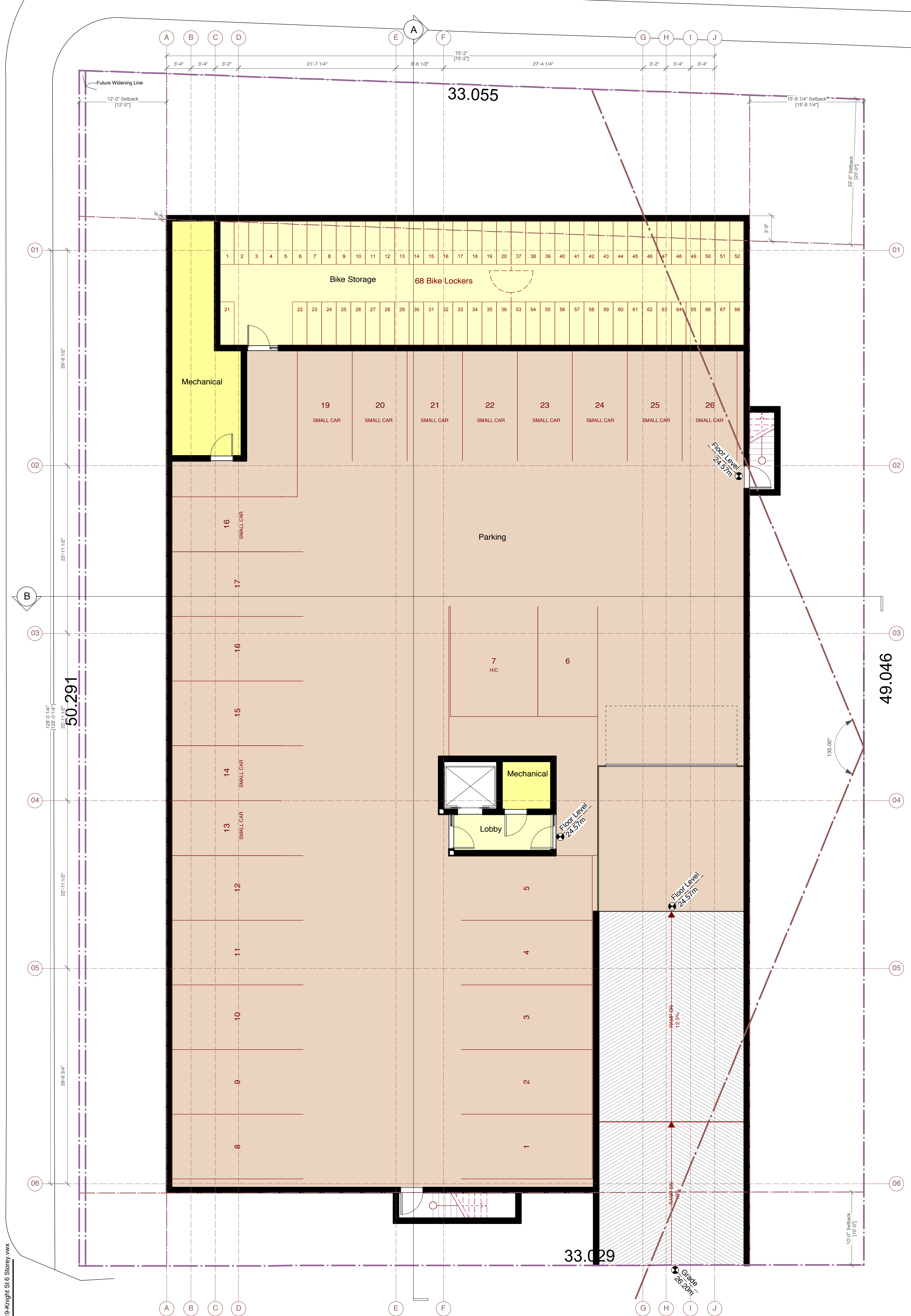
1 Parking Level
