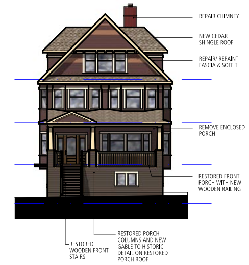
SOUTH ELEVATION
