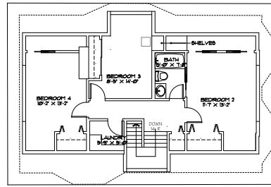
PROPOSED UPPER FLOOR PLAN
