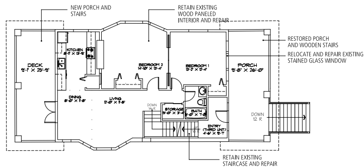
PROPOSED SECOND FLOOR PLAN
