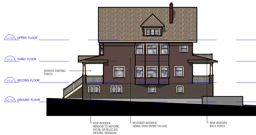
EAST ELEVATION
