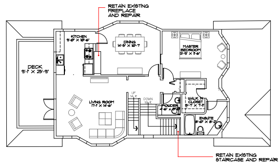
PROPOSED THIRD FLOOR PLAN
