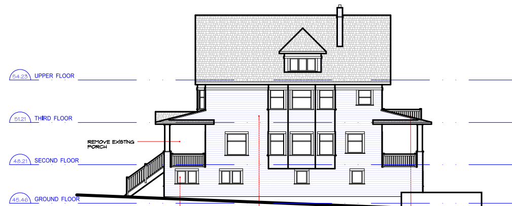
EAST ELEVATION
