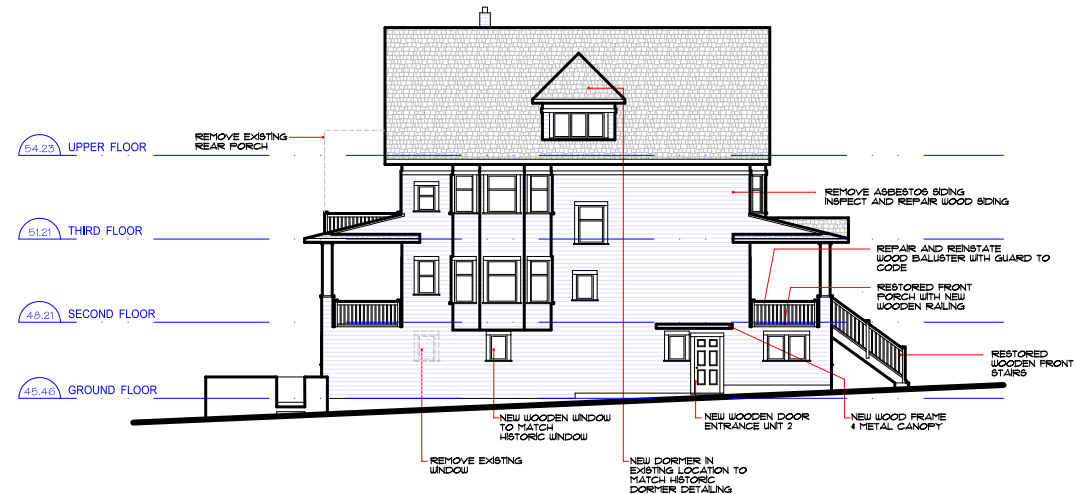
WEST ELEVATION
