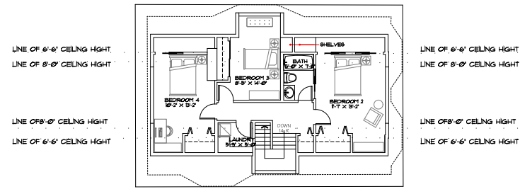
PROPOSED UPPER FLOOR PLAN
