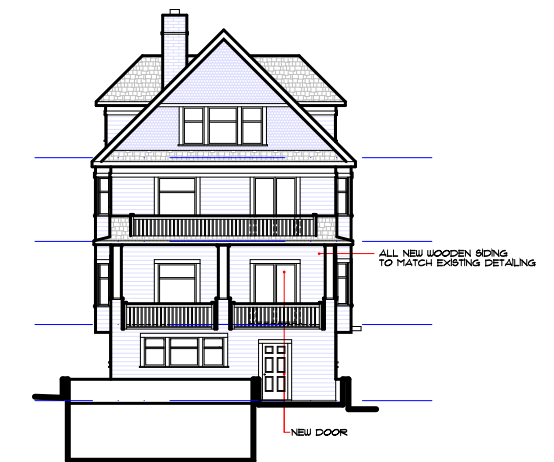
NORTH ELEVATION
