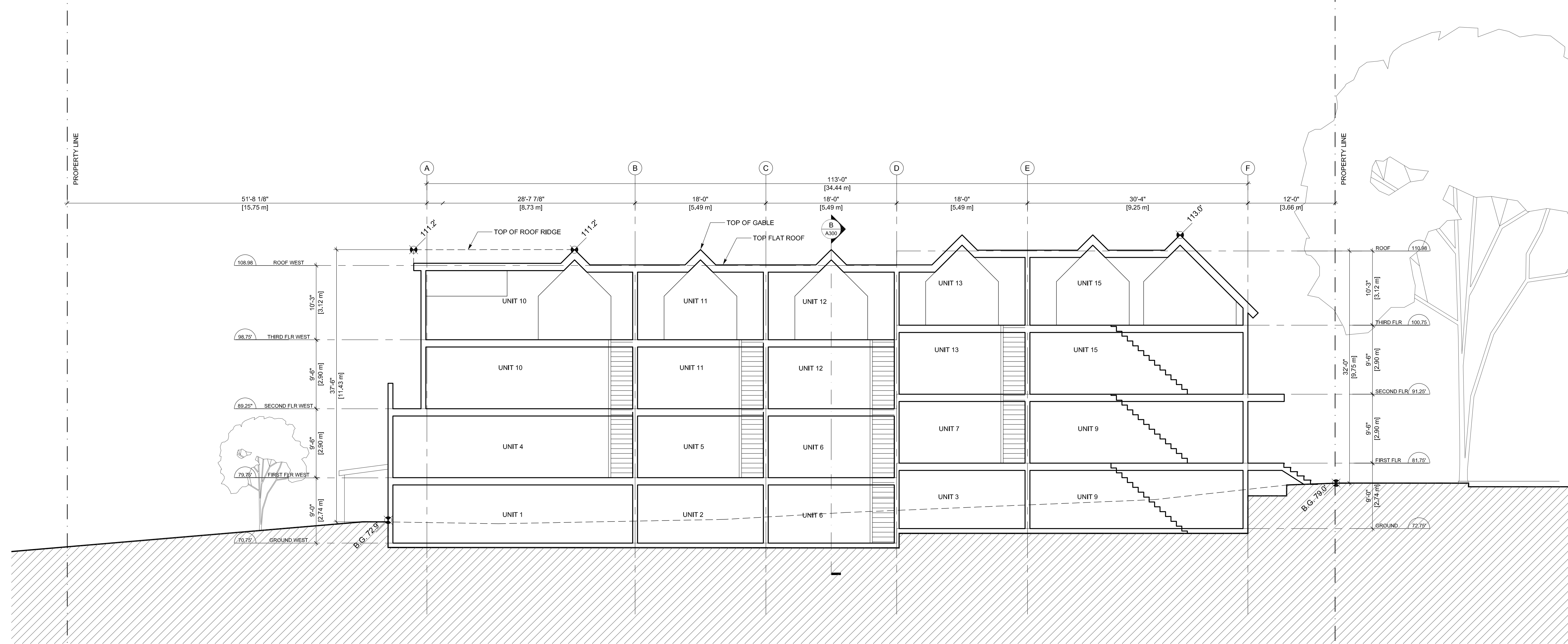
A-A WEST-EAST BUILDING SECTION A301 1/8" = 1'-0"
