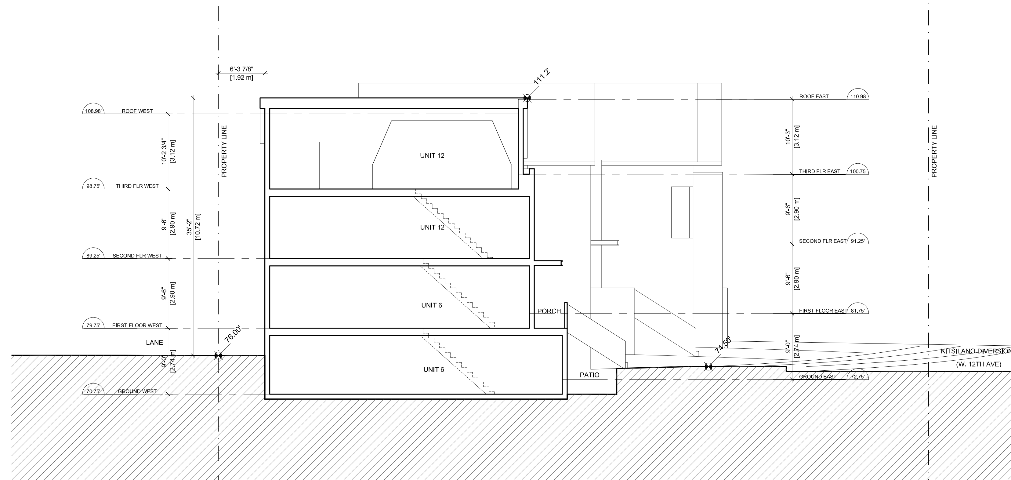
B-B NORTH-SOUTH BUILDING SECTION A301 1/8" = 1'-0"
