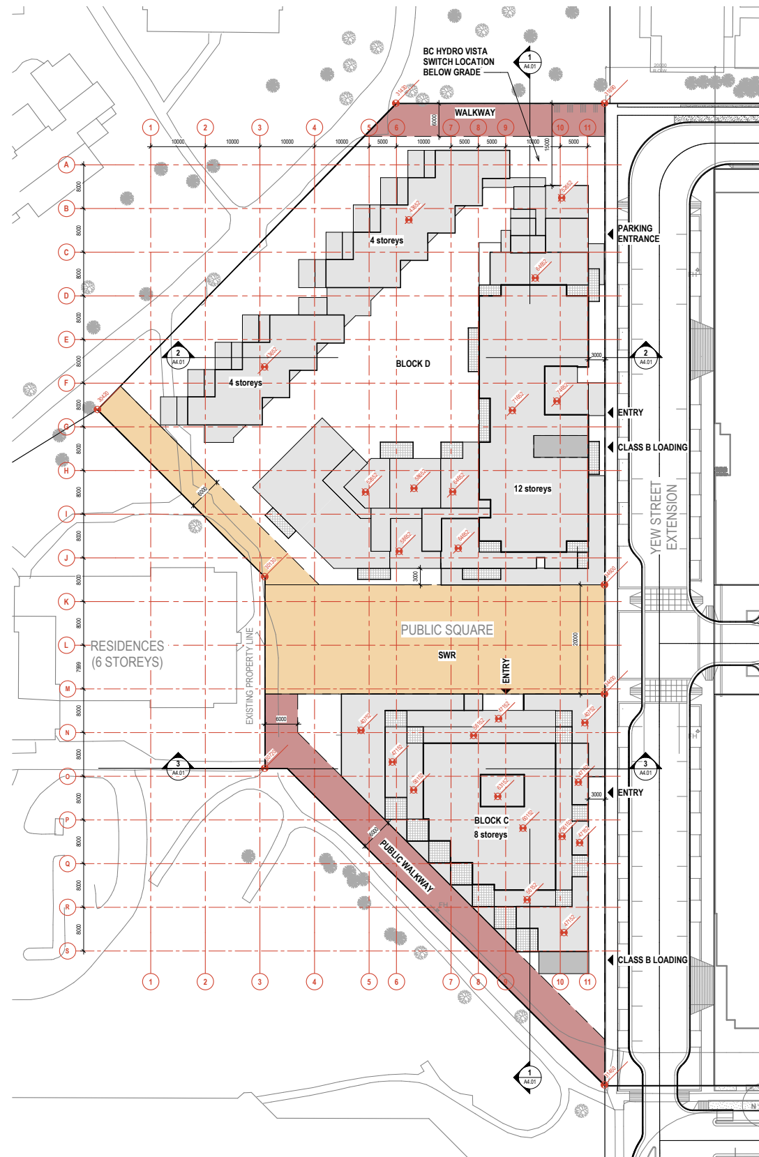
Technical Site Plan
