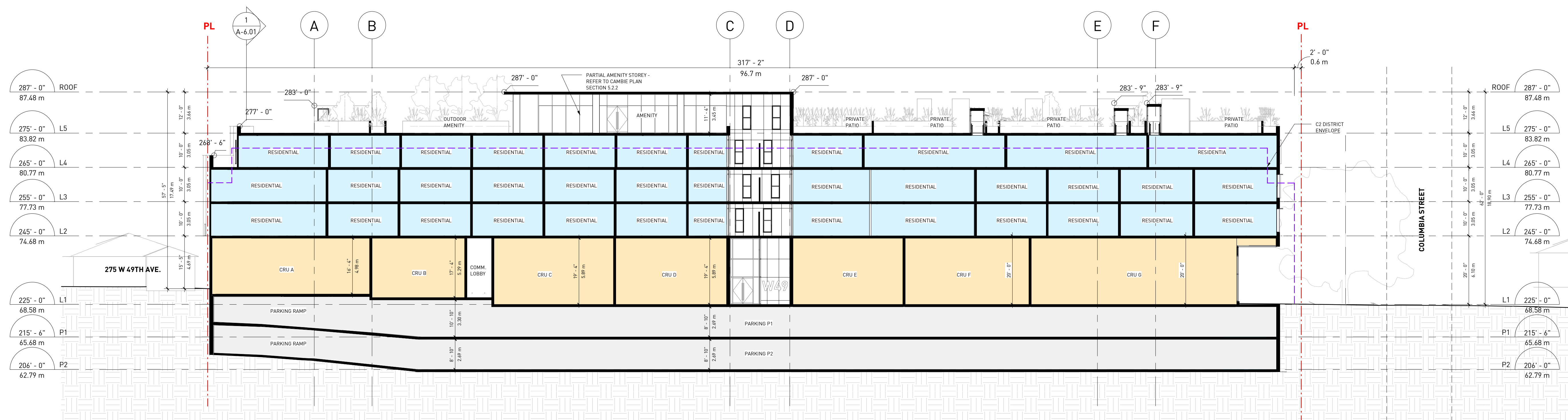
1 SECTION 1 1/16" = 1'-0"
