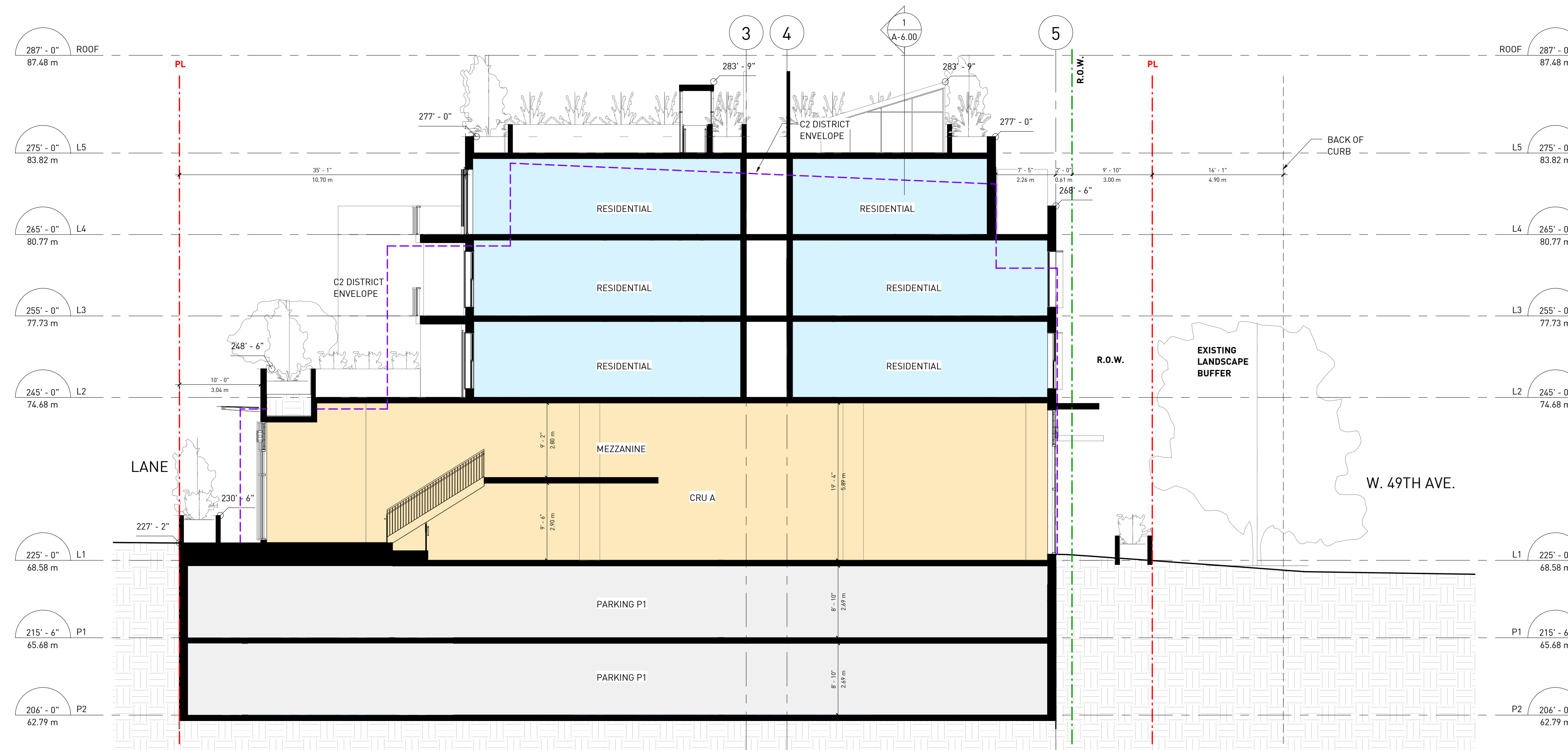
2 SECTION 3 ref. A-1.00
