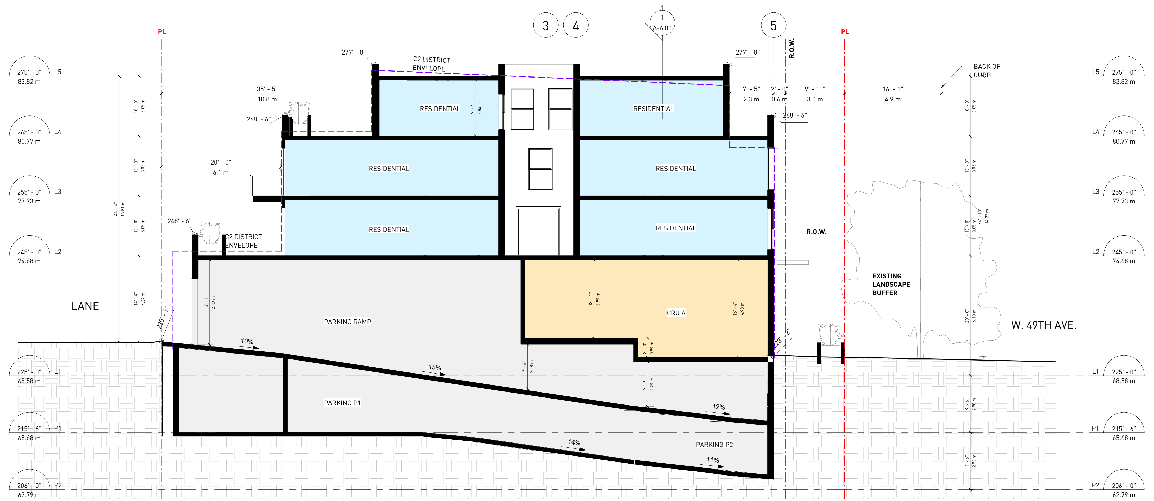
1 SECTION 2 ref. A-1.00
