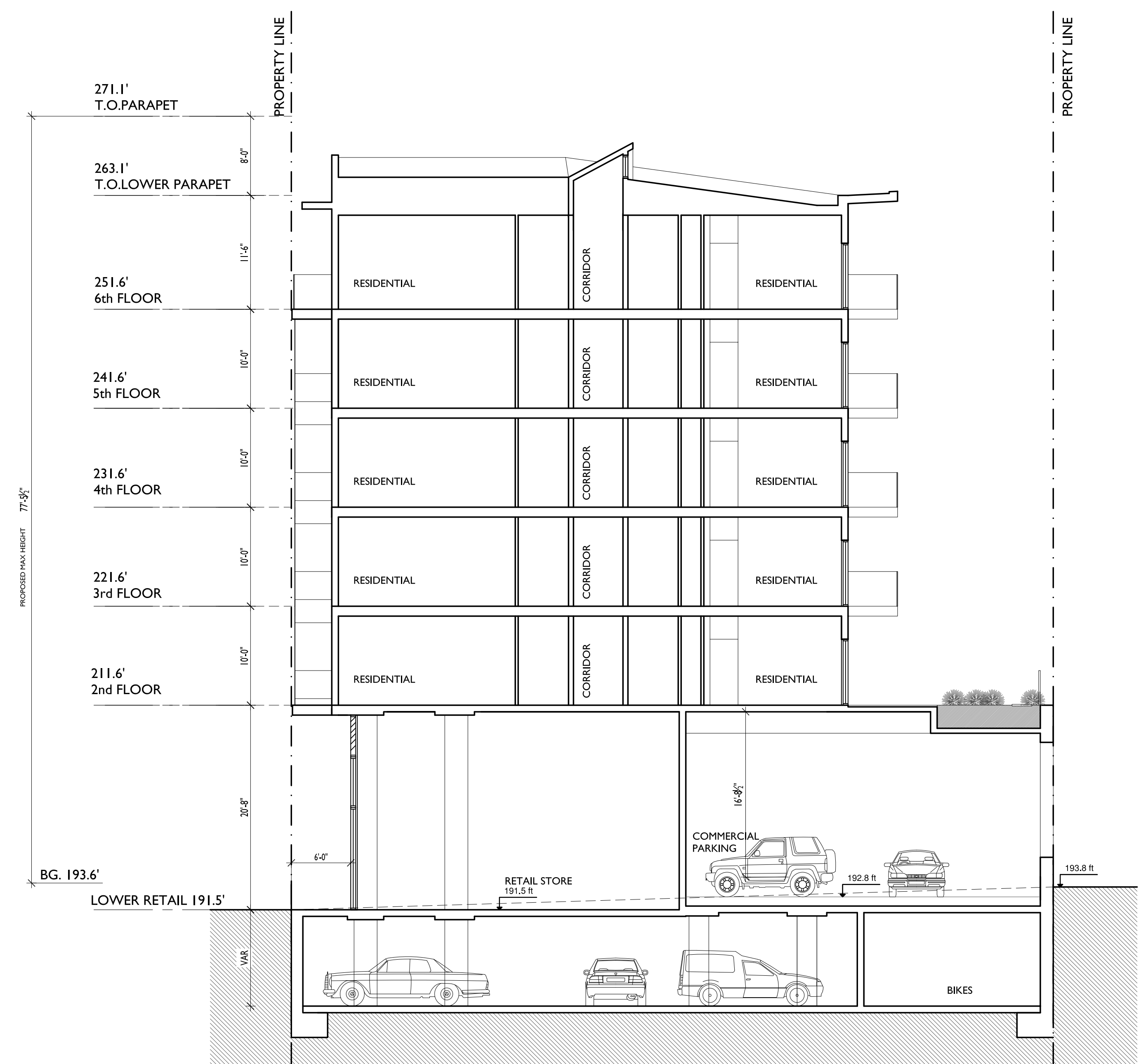
SECTION C-C
