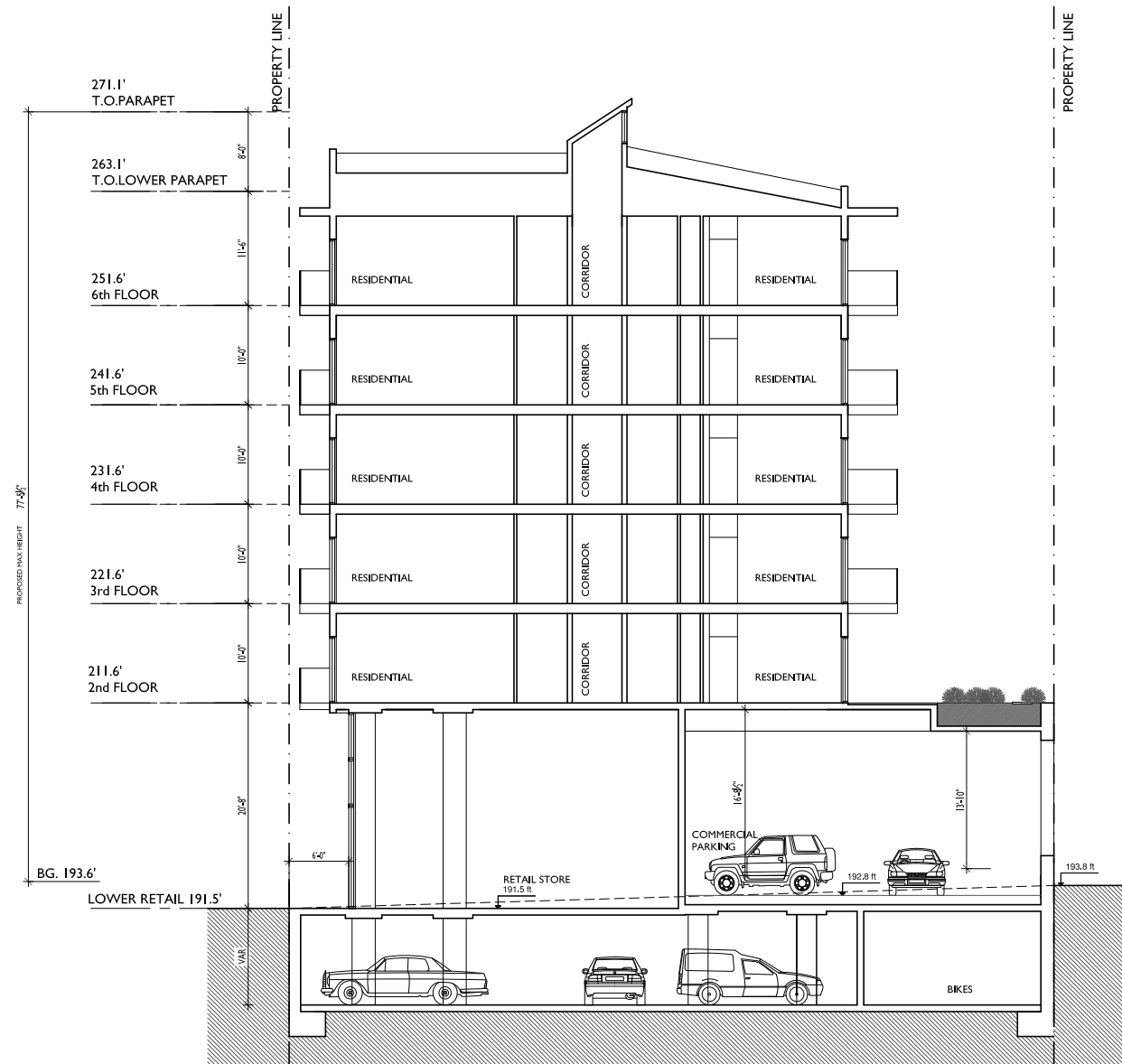
SECTION C-C
