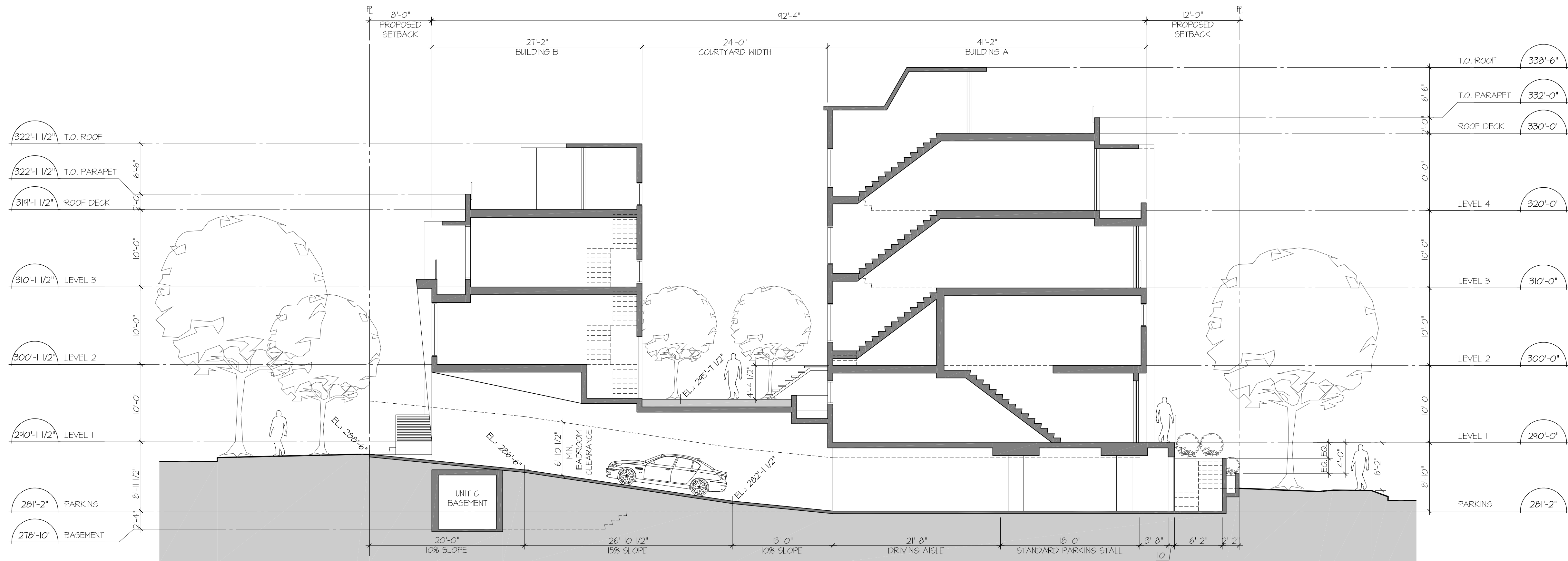
2 SECTION BB - PARKING RAMP 1/8" = 1'-0"
