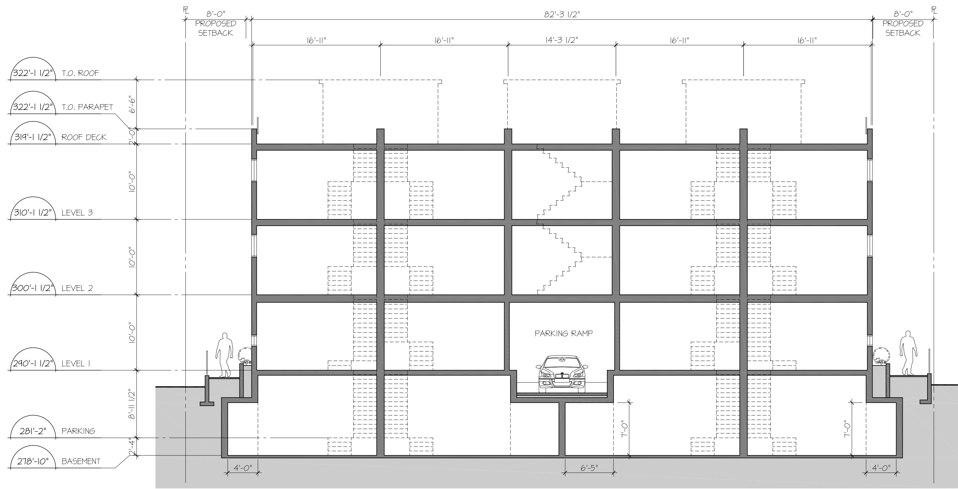
1 SECTION CC - BUILDING B 1/8" = 1'-0"
