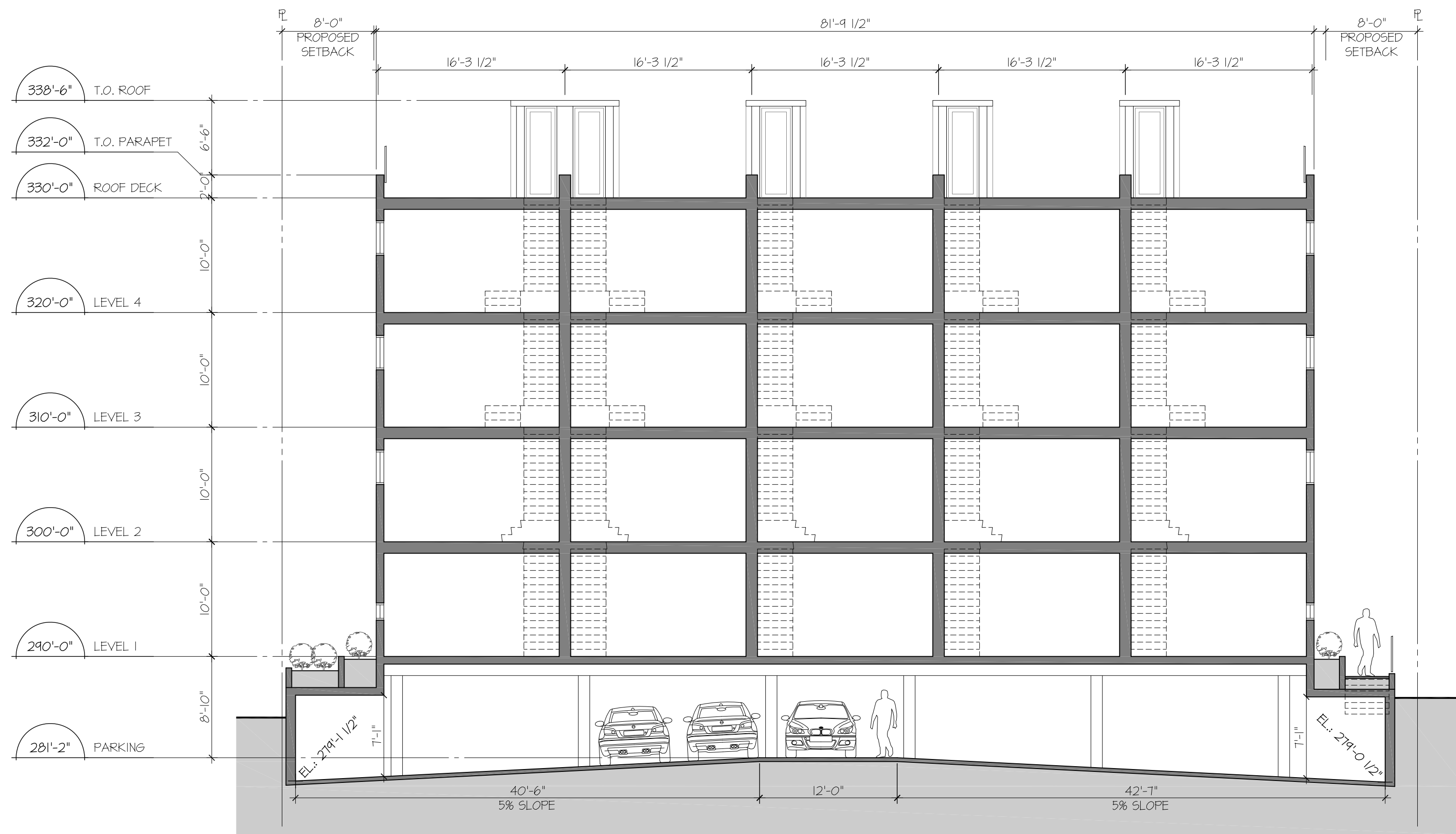
2 SECTION DD - BUILDING A 1/8" = 1'-0"
