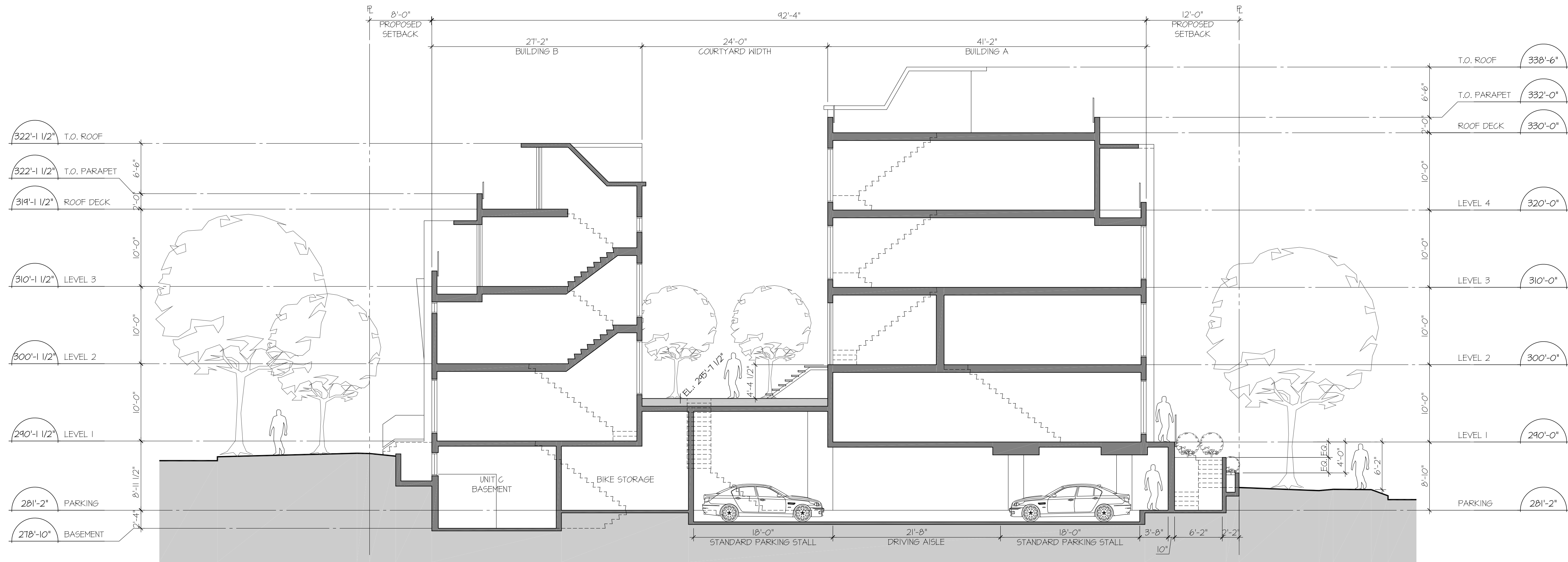
1 SECTION AA 1/8" = 1'-0"
