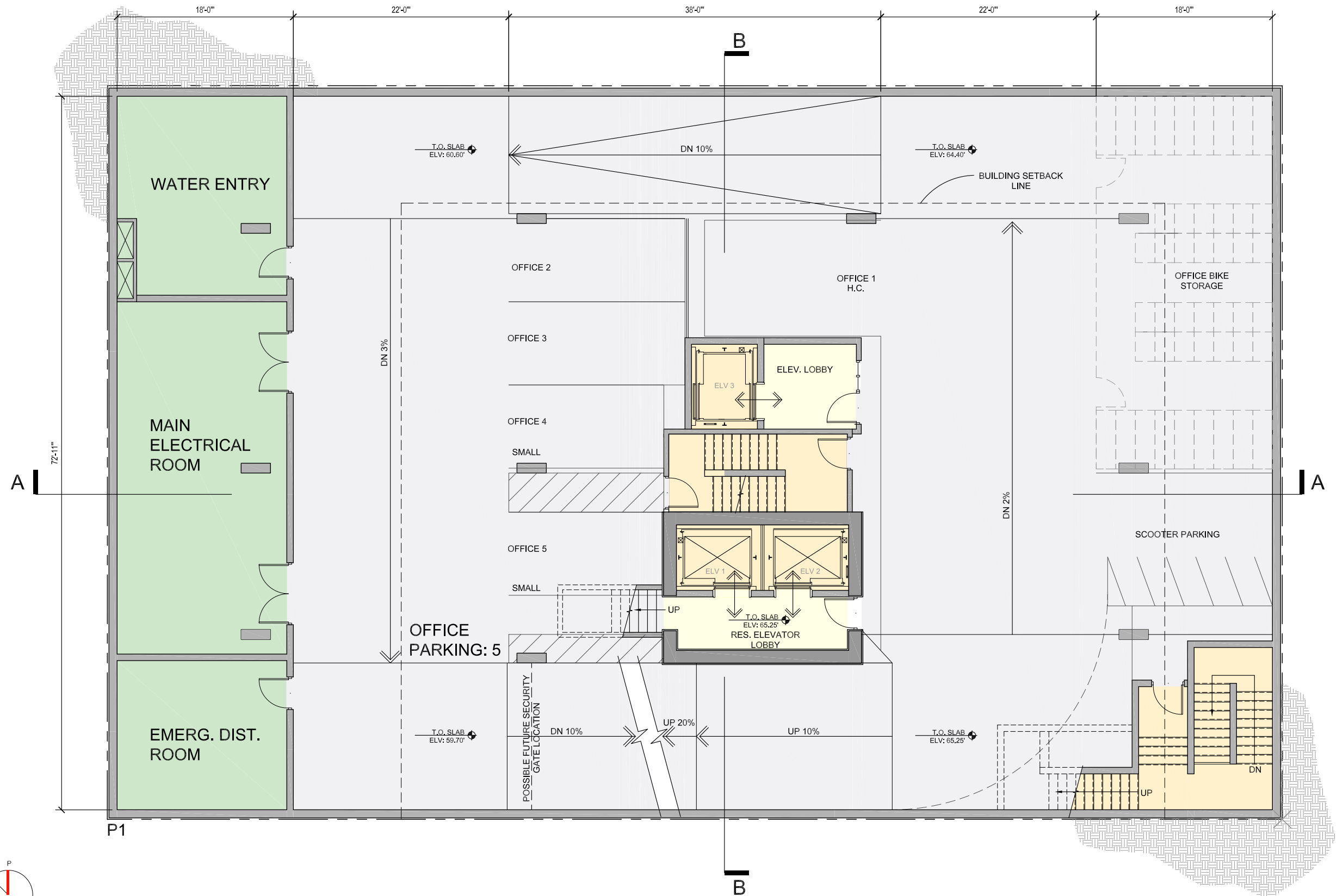
LEVEL P1 - BELOW GRADE PARKING PLAN
