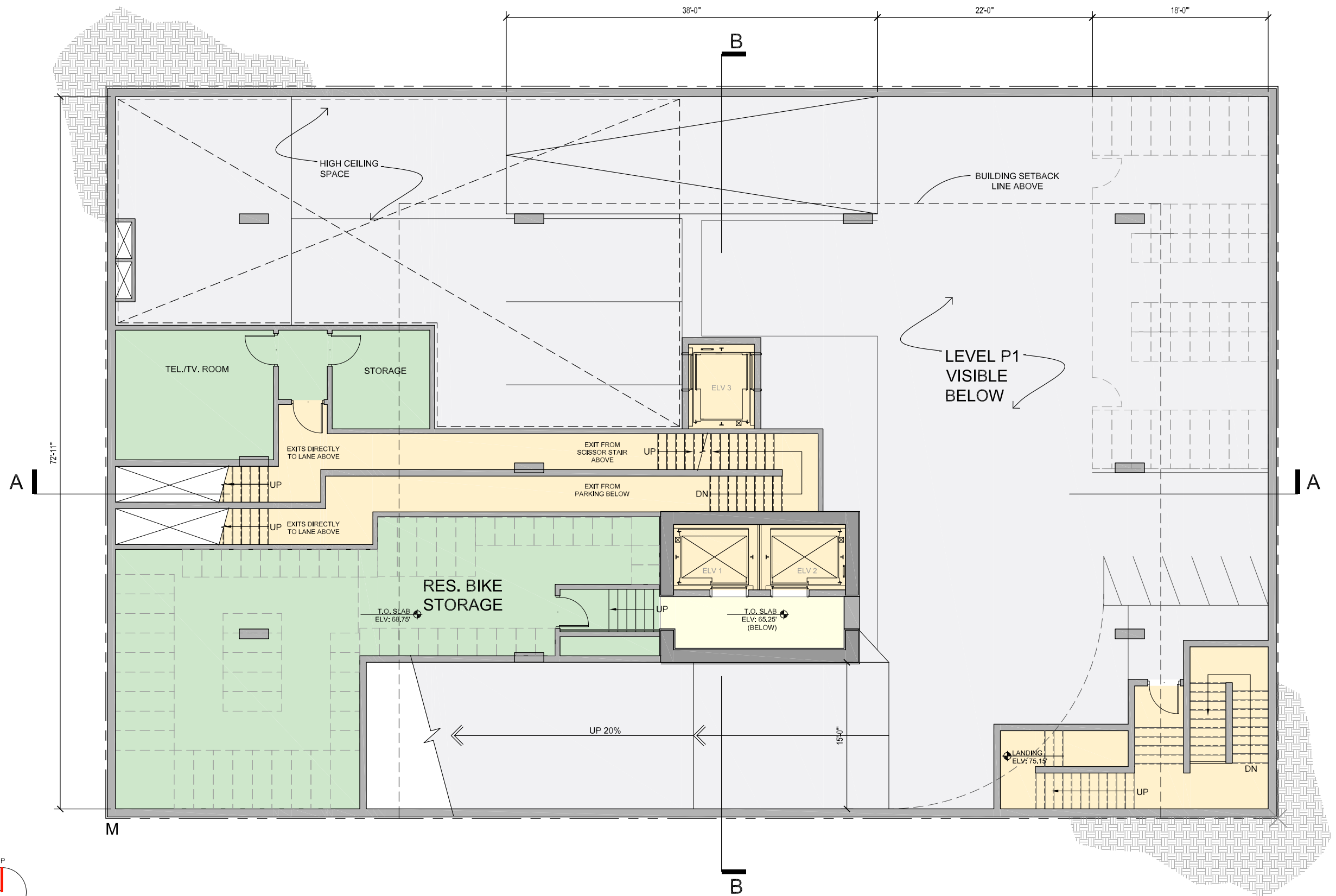
BELOW GRADE MEZZANINE LEVEL PLAN
