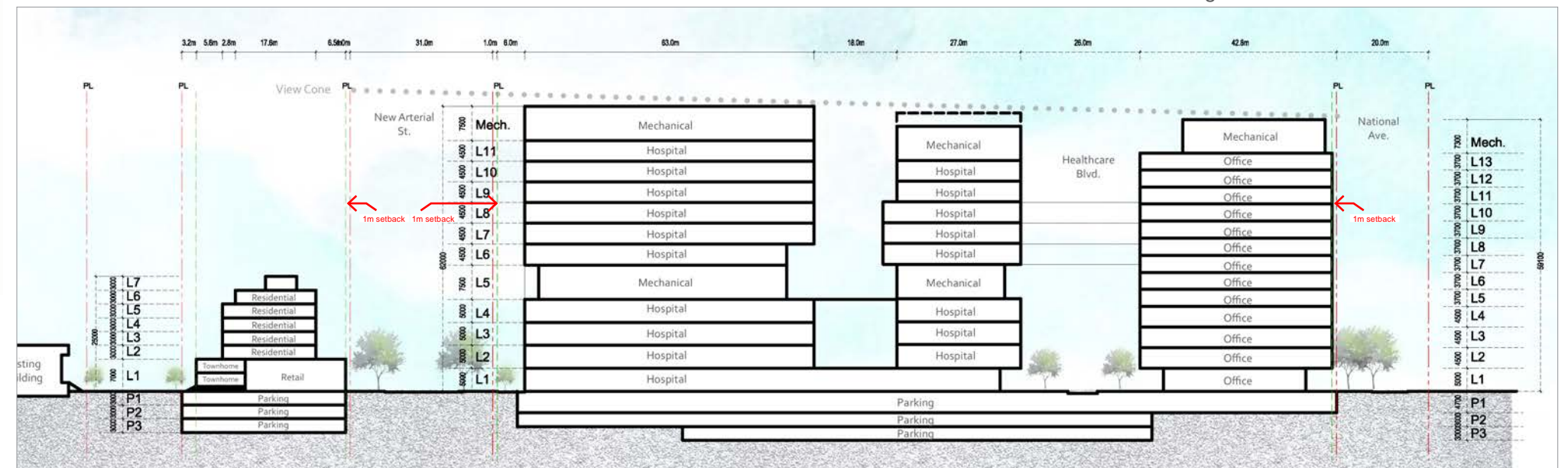
Figure 2-21: Indicative Cross Section AA
