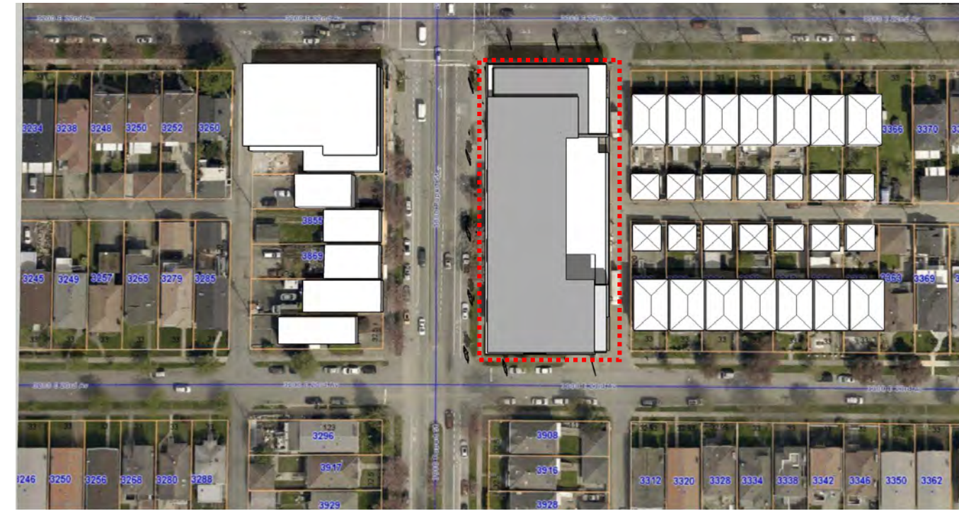
SUMMER SOLSTICE - 12PM
