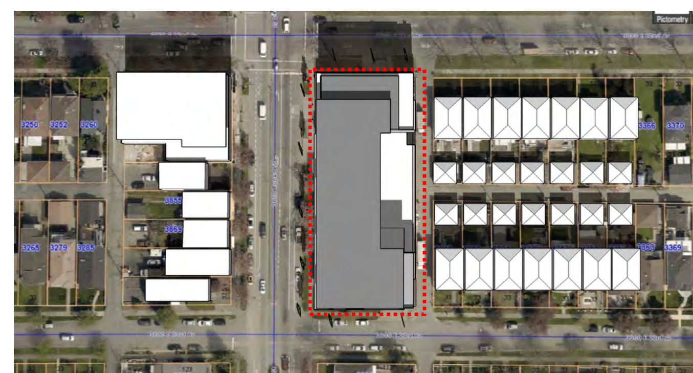
AUTUMN EQUINOX - 12PM
