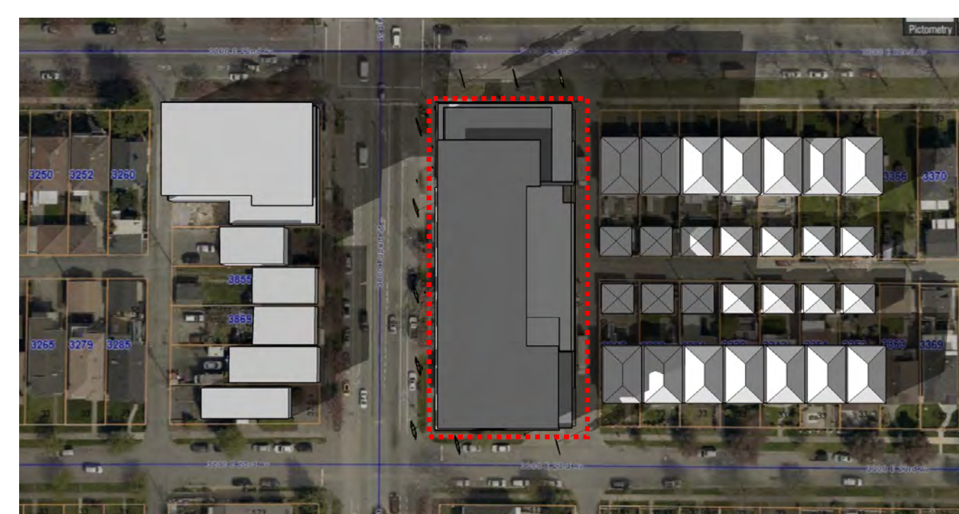
AUTUMN EQUINOX - 4PM
