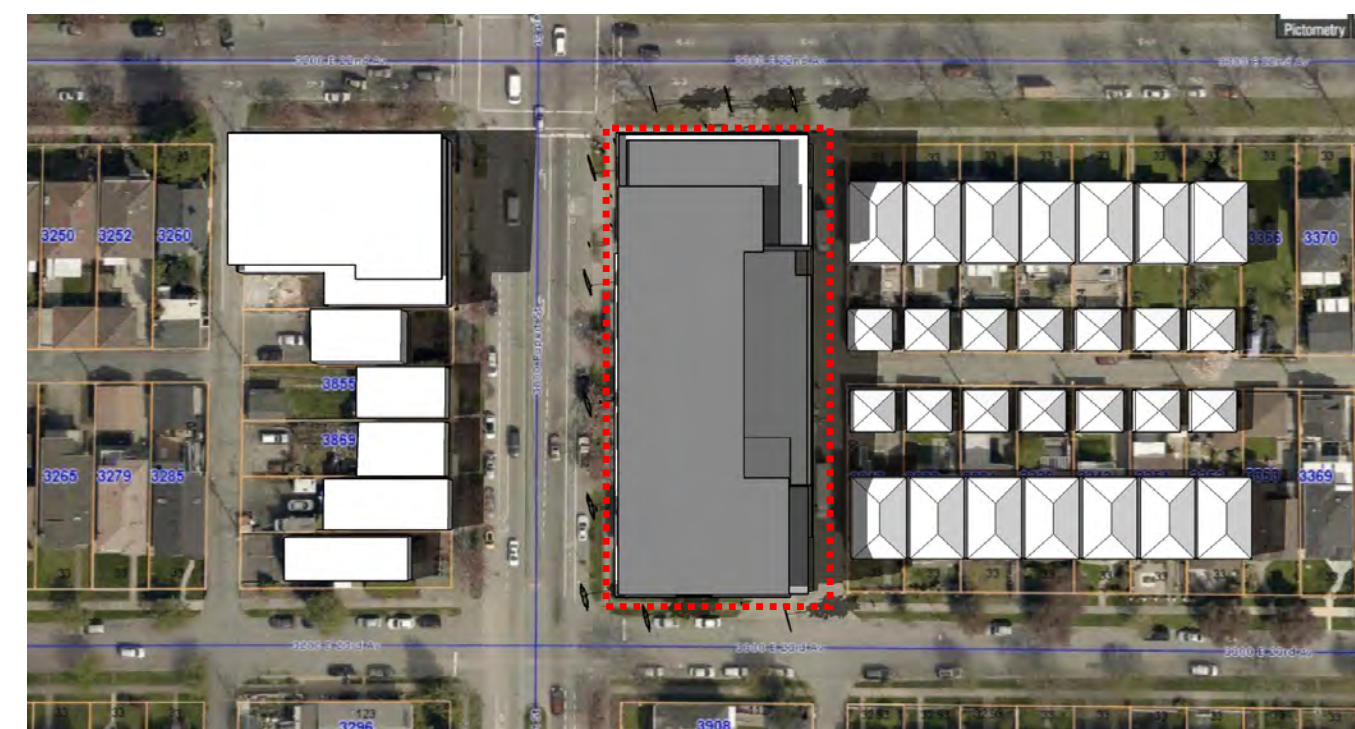
SUMMER SOLSTICE - 4PM
