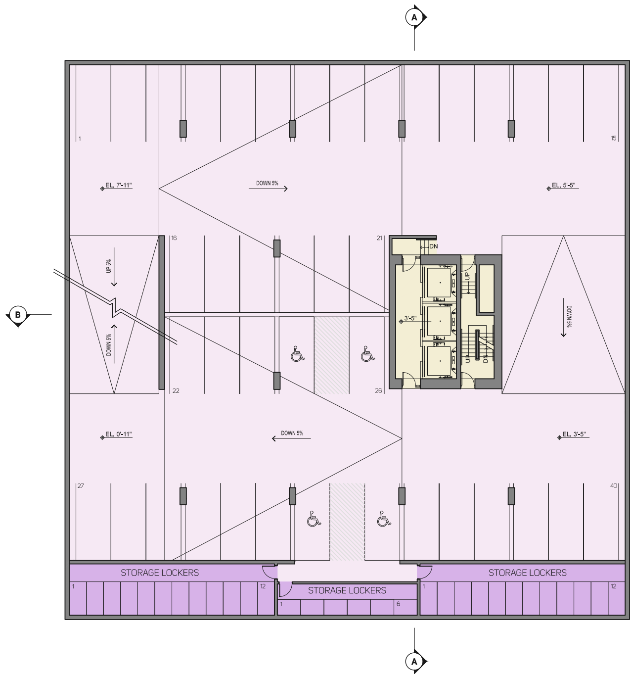
4.2.3 P3 - Parking and Storage
