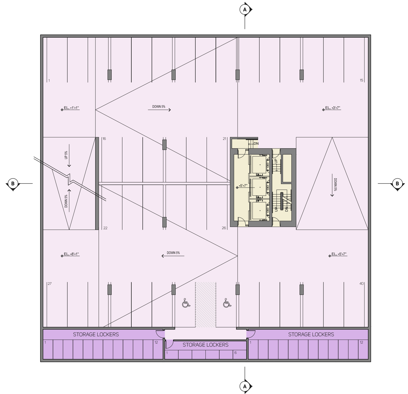
4.2.2 P4 - Parking and Storage
