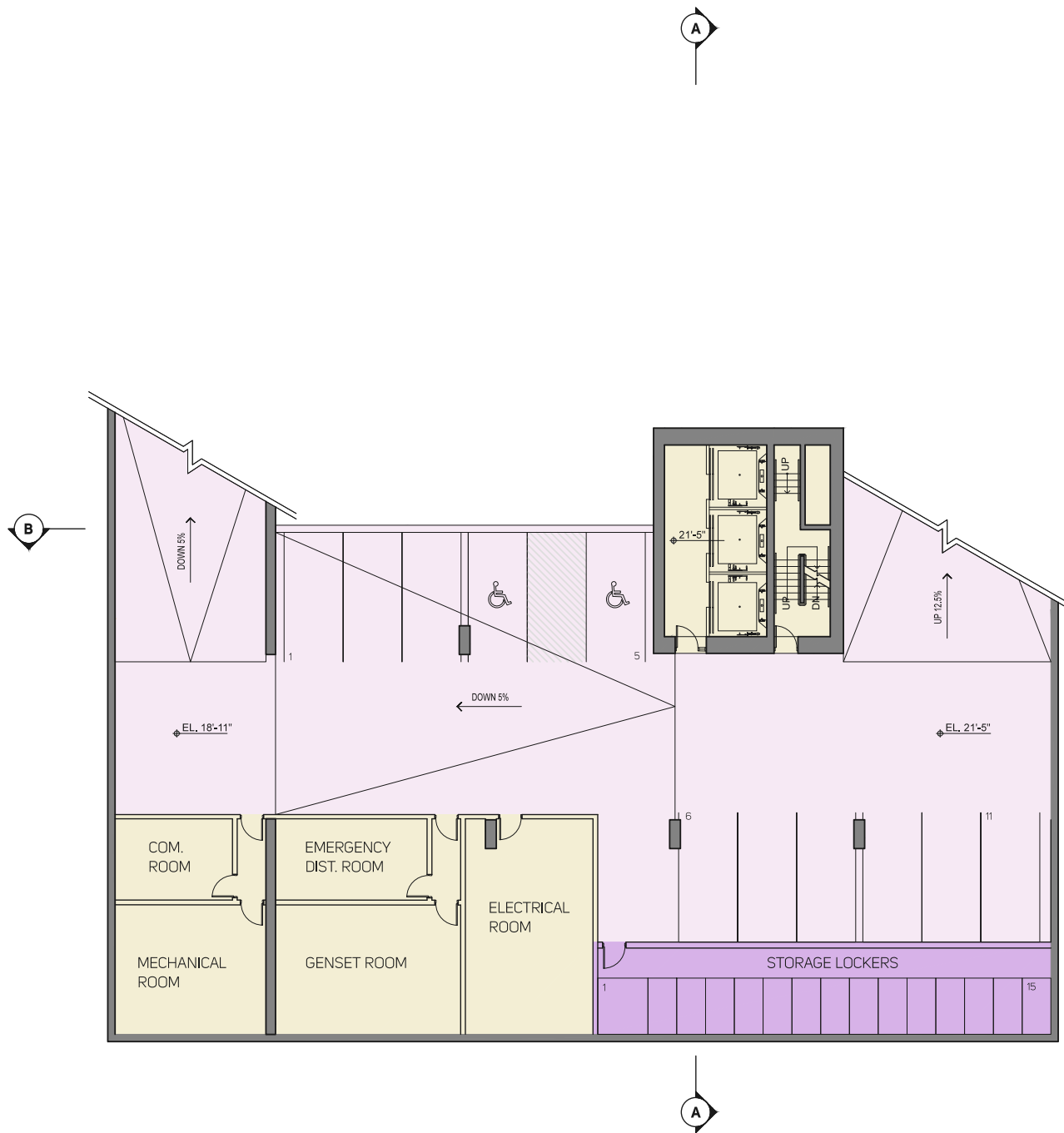
4.2.5 P1 Lower - Parking, Storage, Services
