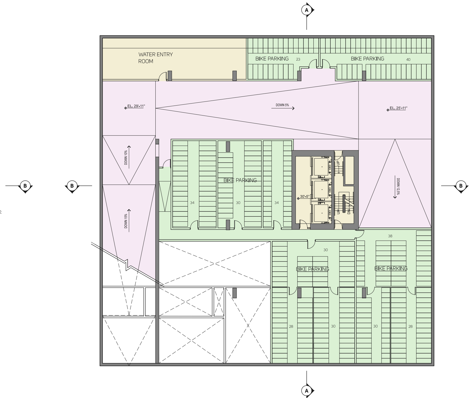
4.2.6 P1 - Bicycle Parking and Services
