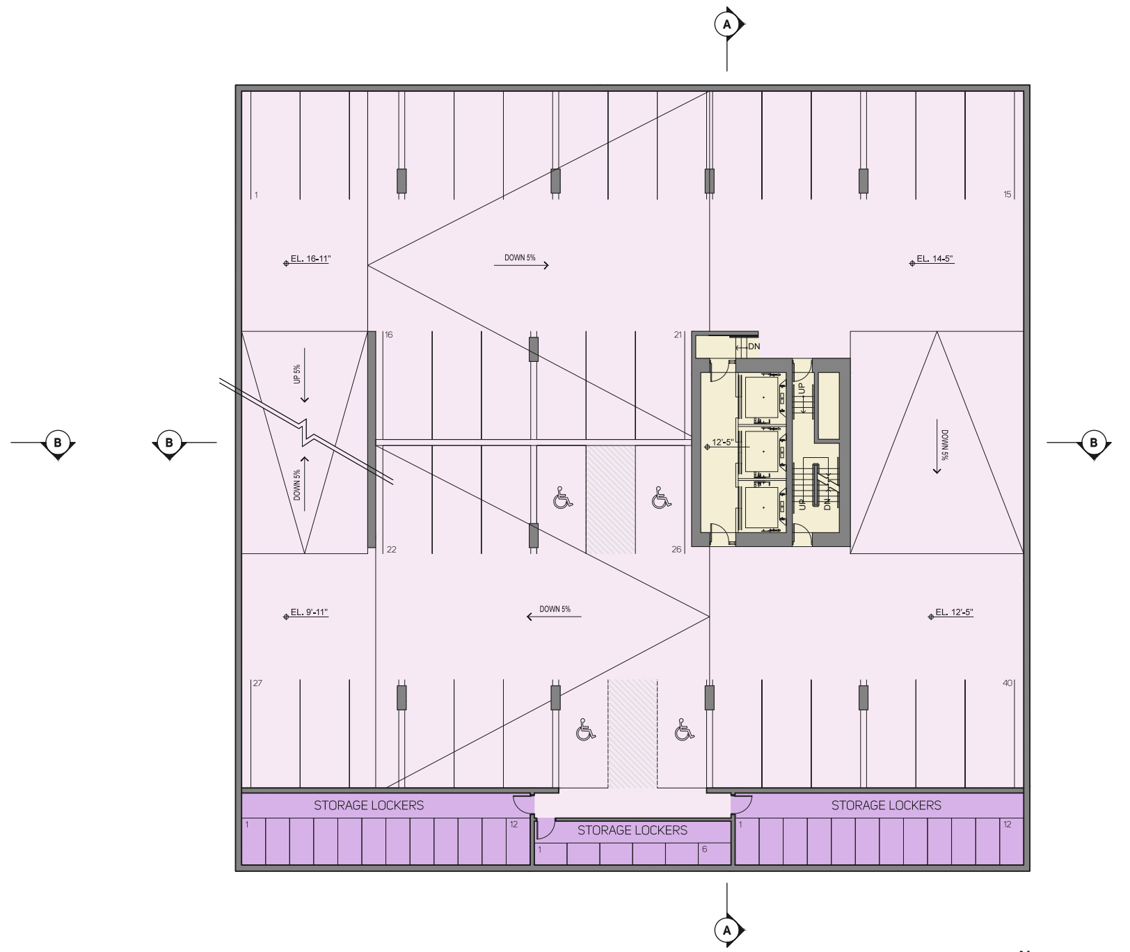
4.2.4 P2 - Parking and Storage
