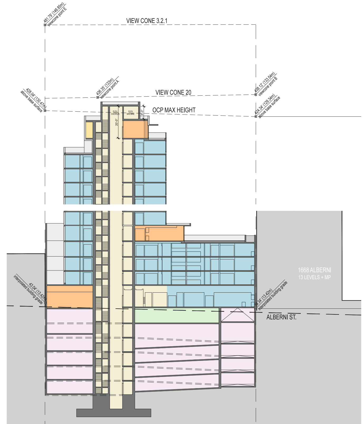
4.4.4 Section B B Detail
