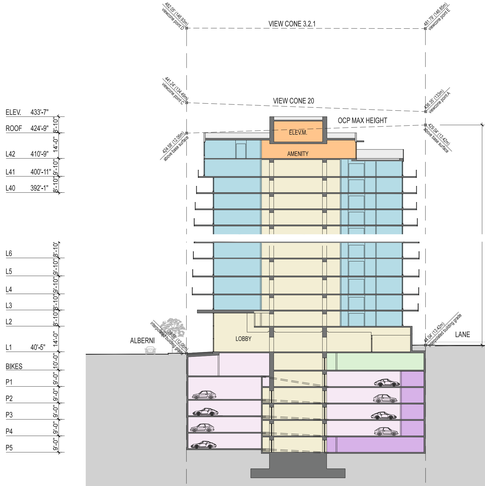
4.4.3 Section A A Detail
