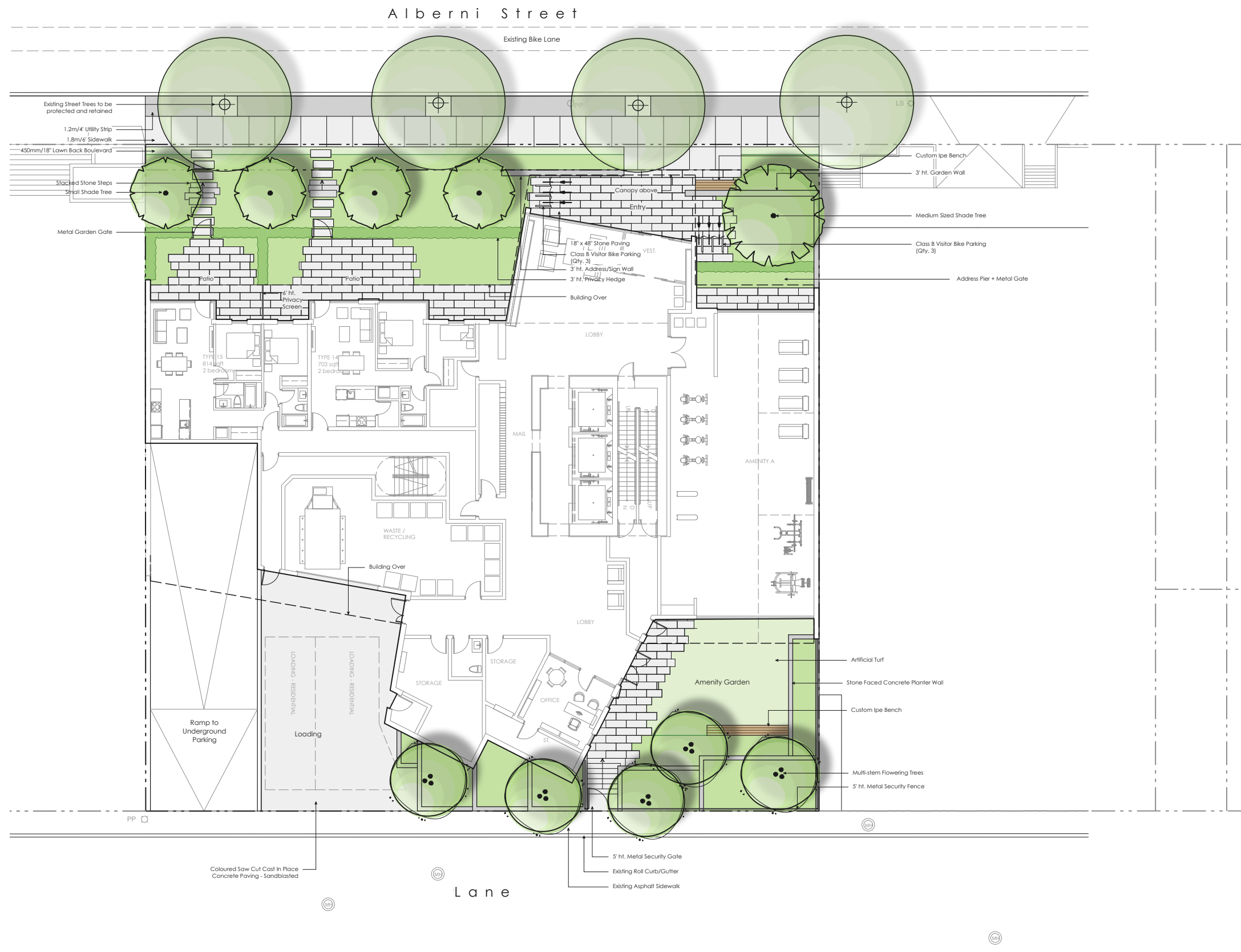
4.3.1 Ground Floor Landscape Plan
