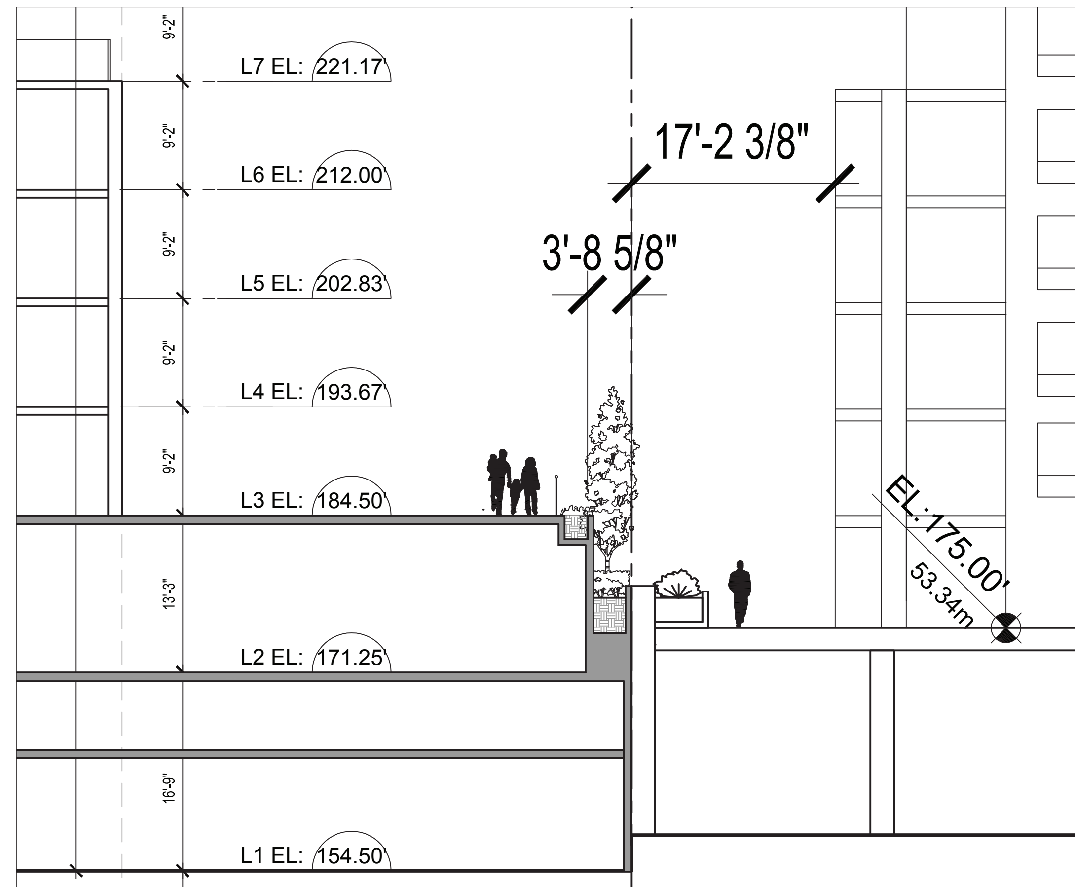
1 SECTION 1 1/8" = 1'-0"
