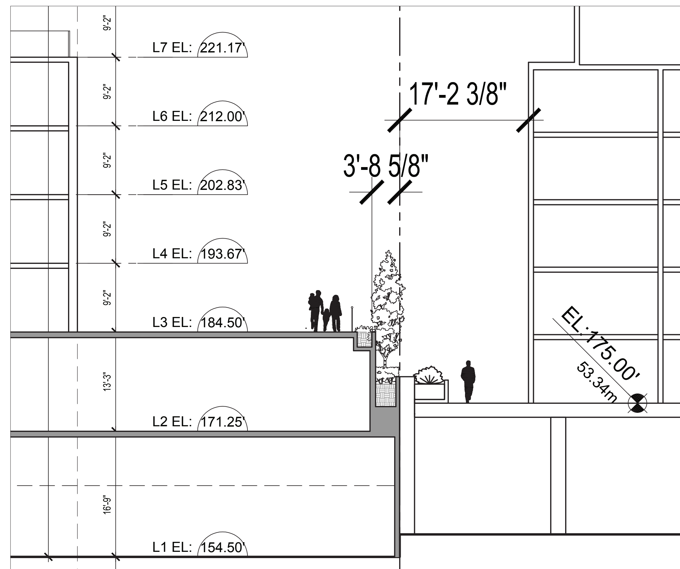
2 SECTION 2 1/8" = 1'-0"
