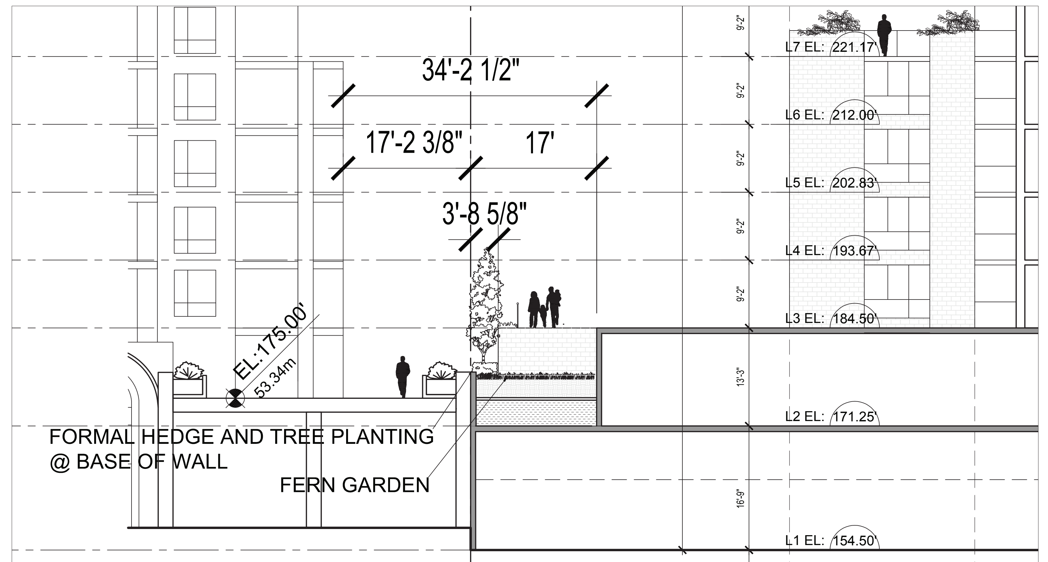
3 SECTION 3 1/8" = 1'-0"
